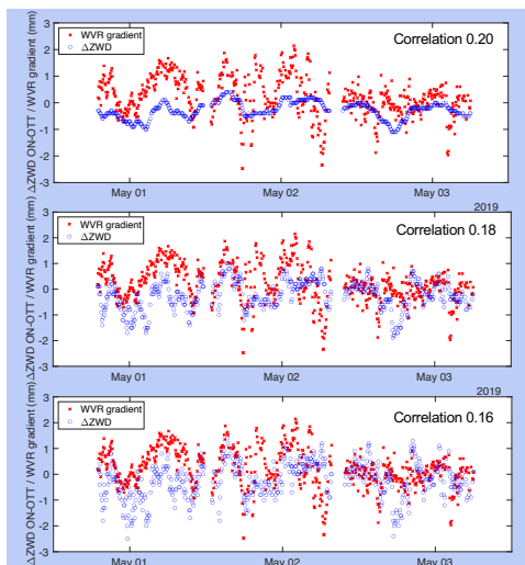
Figure 2. An example of estimated \Delta ZWD (ON–OTT) and WVR gradients mapped on to the ON–OTT baseline for two contiguous experiments. Constraints used are 50 ps/h (top), 200 ps/h (middle), and 350 ps/h (bottom).
