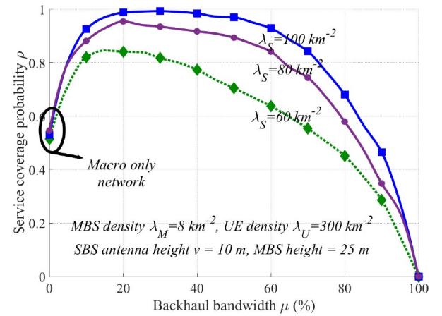
FIGURE 12. Service coverage probability as a function of the backhaul bandwidth allocation percentage \mu in (11) for a dense network, no rain, R_{\text{th}} = 100 \text{ Mbps} , and P_{\text{MBS}}, P_{\text{SBS}}, P_{\text{UE}} = (40, 24, 0) \text{ dBm} .
