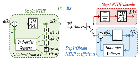
Fig. 1: Block diagram of NTHP-Volterra equalizer.
