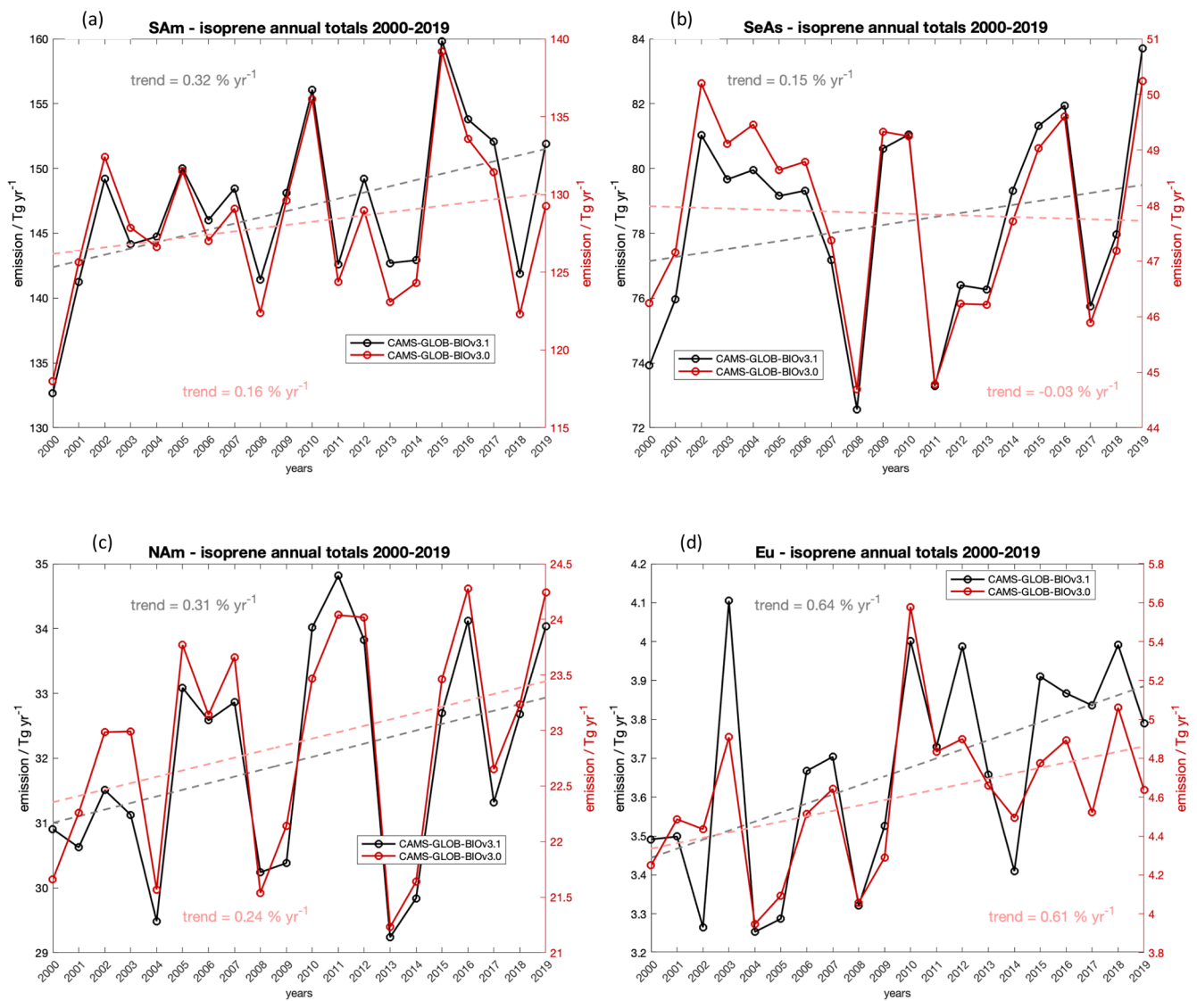
Figure 4. Comparison of isoprene annual totals from CAMS-GLOB-BIOv3.0 and v3.1 in (a) South America, (b) Southeast Asia and Indonesia, (c) North America, and (d) Europe with linear trend for each dataset (dashed line and trend value in % yr -1 ).
