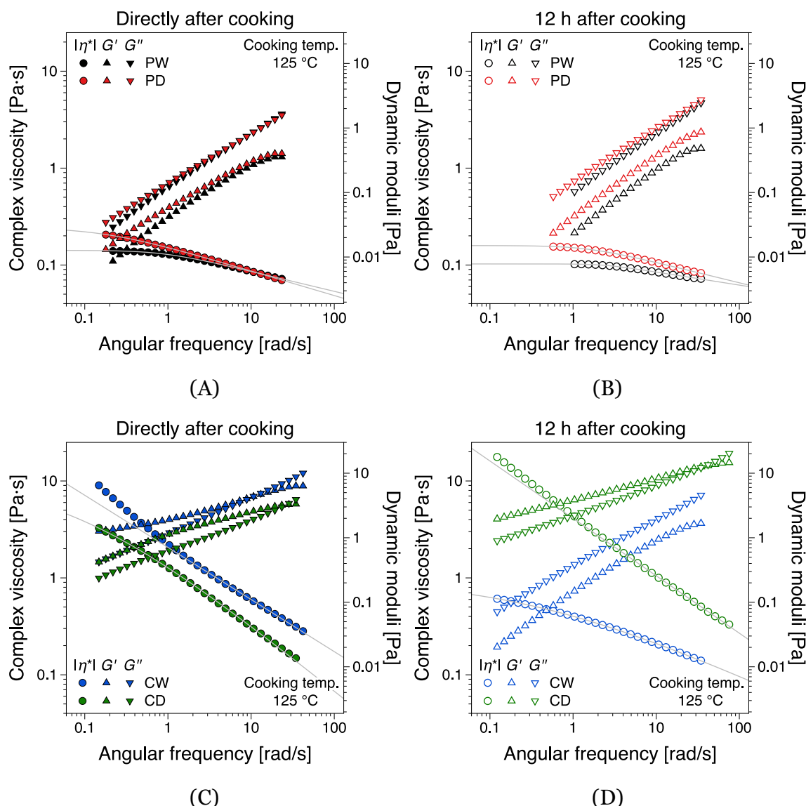
Fig. 2. Frequency sweep tests ( \gamma_0 = 18\% , 50^\circ\text{C} ) of jet-cooked cationic starch solutions ( 125^\circ\text{C} , 3.5\text{ wt\%} , I = 3\text{ mM} ) directly after cooking (A, C) and after 12 h of storage at room temperature (B, D). The continuous lines are complex viscosity (magnitude) function fits according to Eqs. (1)–(2).
