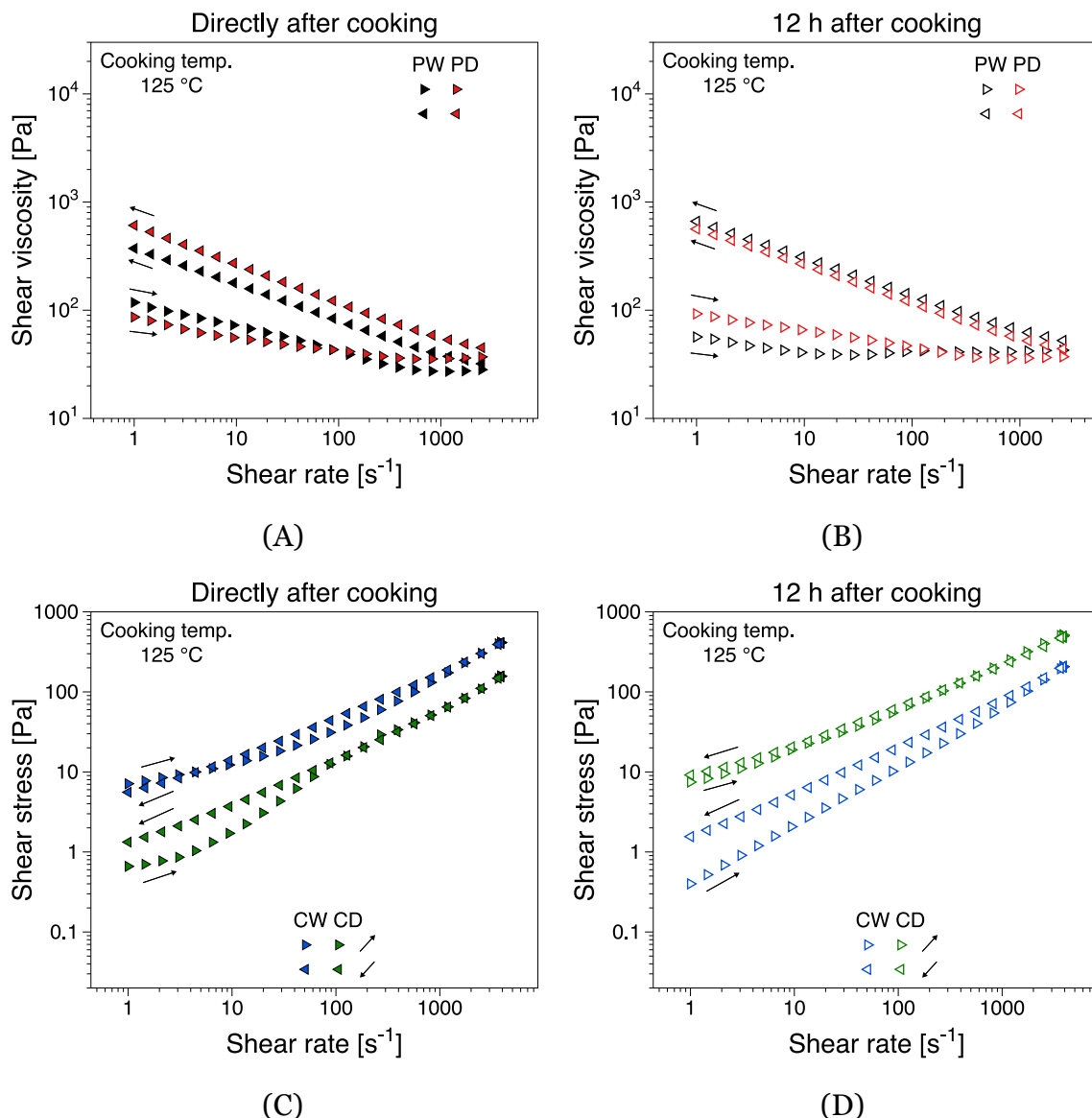
Fig. 3. Hysteresis loop flow curves (50 °C) of jet-cooked cationic starch solutions (125 °C, 3.5 wt%, I = 3 mM) directly after cooking (A, C) and after 12 h of storage at room temperature (B, D).
