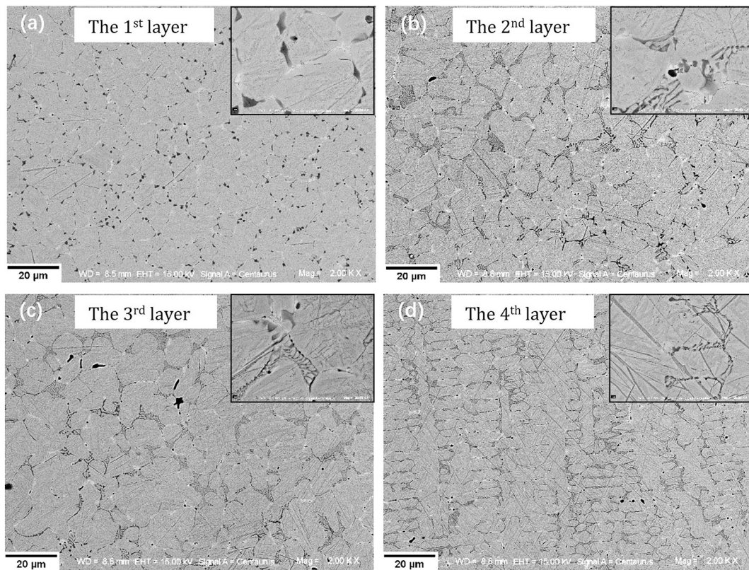
Fig. 5. Comparison of the microstructure from different deposited layers: (a) the 1st layer adjacent to substrate, (b) the 2nd layer, (c) the 3rd layer, (d) the 4th layer (top).
