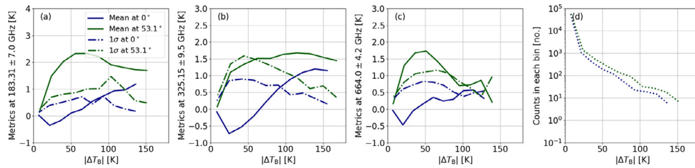
Fig. 11. For the realistic cloud and precipitation scenarios, statistics describing the differences in the cloud impact between ARTS and RTTOV, i.e., \Delta T_{B, \text{ARTS}} - \Delta T_{B, \text{RTTOV}} , binned as a function of the cloud impact ( \Delta T_B in absolute values) for two earth incident angles, i.e., 0^\circ (solid lines) and 53.1^\circ (dashed lines): (a) at 183.31 \pm 7.0 GHz, (b) at 325.15 \pm 9.5 GHz, (c) at 664.0 \pm 4.2 GHz, while in (d) the number of observations binned by the cloud impact is highlighted (same over all frequencies).
