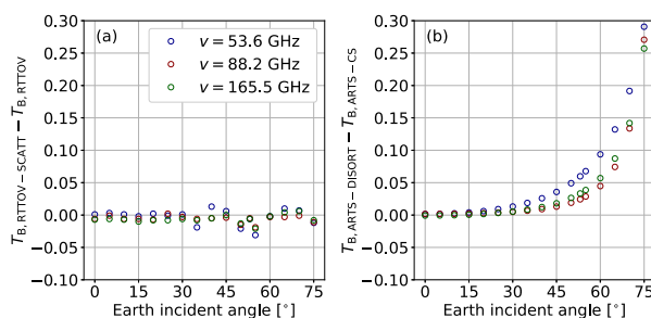
Fig. B.13. Clear-sky consistency between clear-sky and scattering solvers as a function of the earth incident angle for the three frequencies of ATMS (Advanced Technology Microwave Sounder) considered in this study: (a) RTTOV vs. RTTOV-SCATT and (b) ARTS in-house clear-sky solver (ARTS-CS) vs. DISORT. Results are presented for the tropical FASCOD profile.
