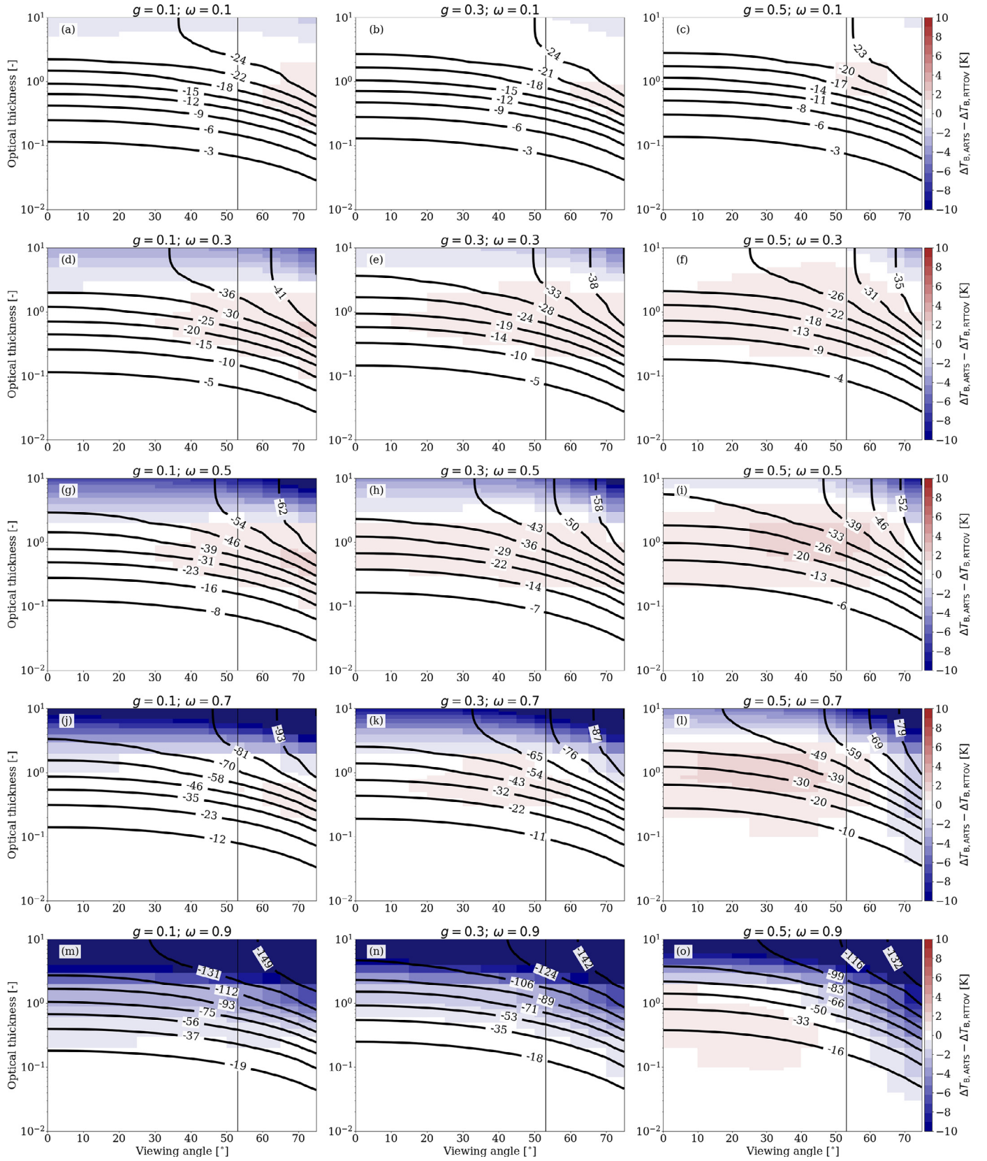
Fig. 4. For the idealized cloudy scenarios, differences in the cloud impact between ARTS and RTTOV, i.e., \Delta T_{B,ARTS} - \Delta T_{B,RTTOV} , as a function of the earth incident angle and the cloud optical thickness for various values of the asymmetry parameter ( g ) and the single scattering albedo ( \omega ). The black contours denote \Delta T_{B,ARTS} , while the black vertical line highlights the earth incident angle of the Ice Cloud Imager (ICI).
