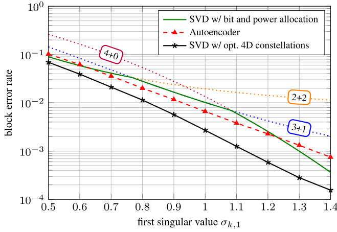
Fig. 6. BLER for the closed-loop MIMO system at SNR = 12 dB over channel matrices with fixed singular values (without retraining). The value of the second singular value is \sigma_{k,2} = 0.5 . The dotted lines correspond to the SVD-based baseline with fixed bit allocation for the two parallel channels.
