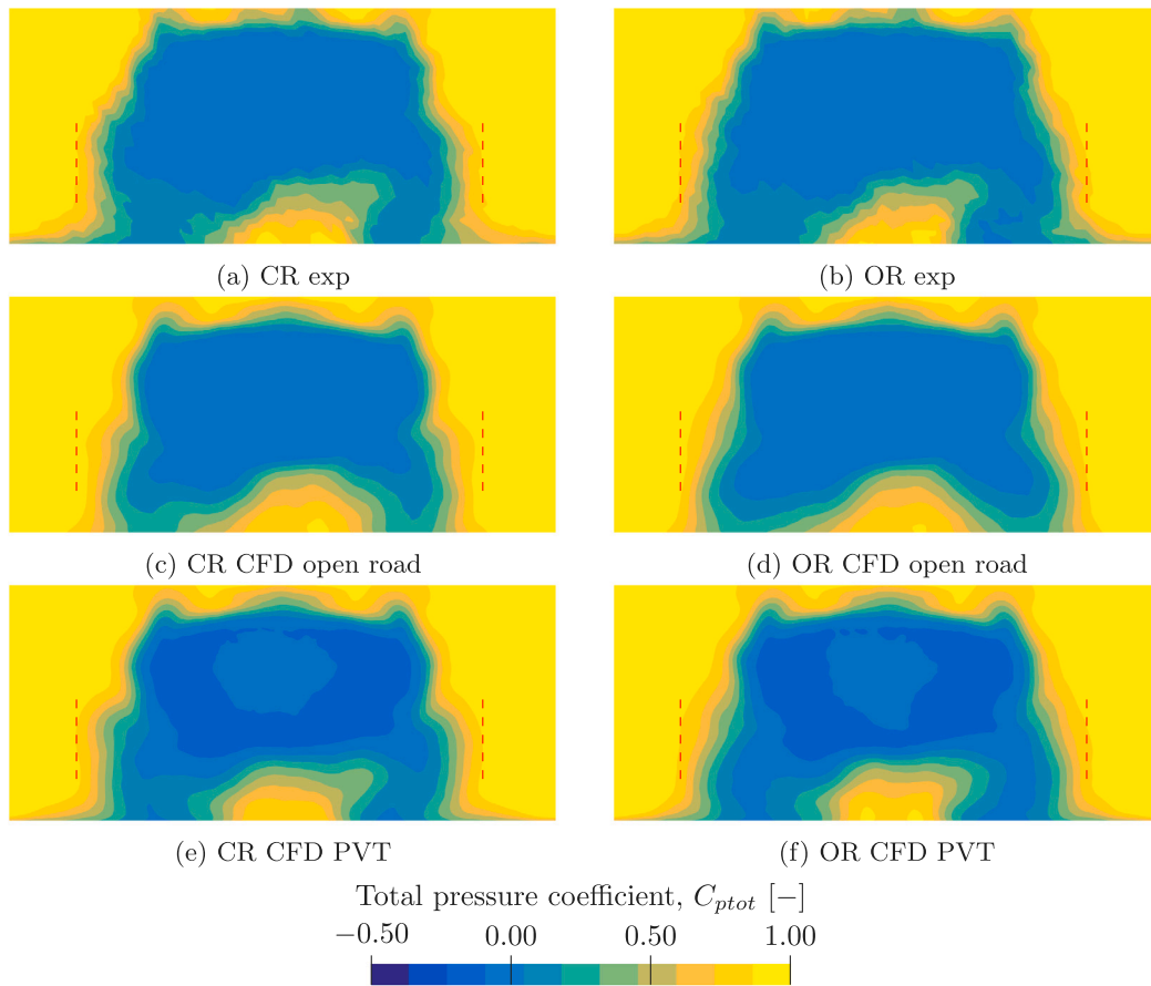
Fig. 25. Total pressure coefficient in the plane x = 4000 mm for the slick tyre with open and closed rims. The lines have been added to assist assessing the width of the separation and are placed at the same location for all cases.
