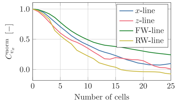
Fig. 8. Two-point correlation for the streamwise velocity along the lines illustrated in Fig. 7.
