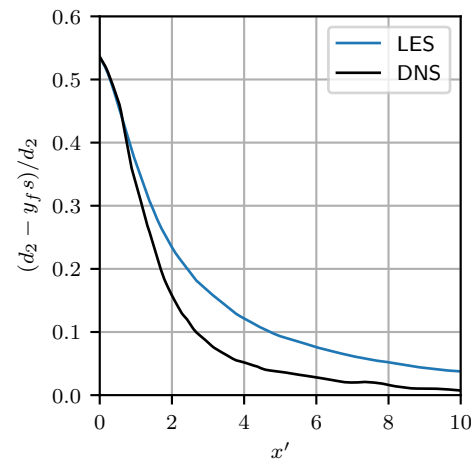
Figure 4. Convergence of the interface height towards d_2 in the benchmark simulation.
