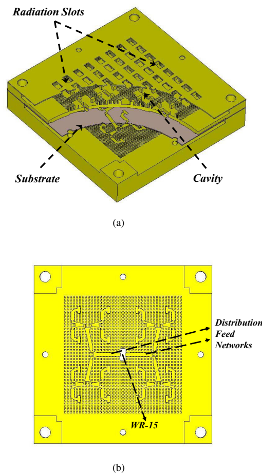
Fig. 1. Configuration for 8 \times 8 slots array antenna. (a) 3-D view for the structure. (b) WR-15 interface view and distribution feed networks.
