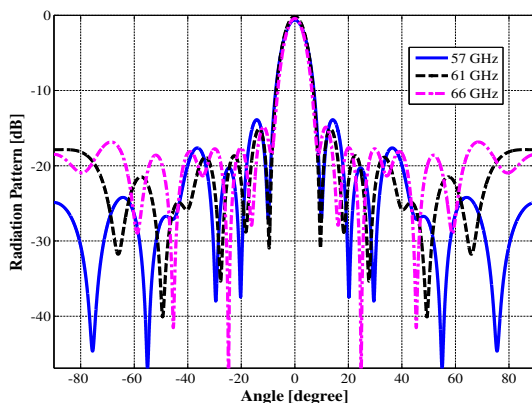
Fig. 3. Simulated E-plane patterns of proposed antenna.
