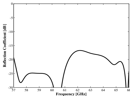
Fig. 2. Simulated reflection coefficient of proposed antenna structure.
