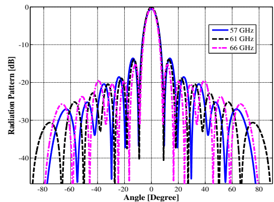
Fig. 4. Simulated H-plane patterns of proposed antenna.
