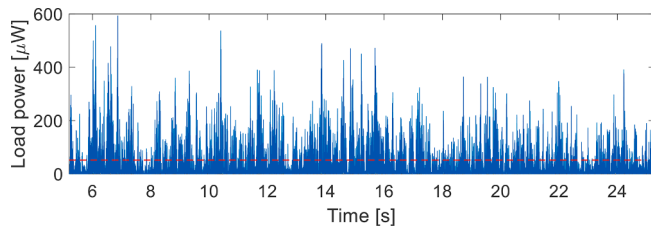
Fig. 15. Simulated load power using measured vibration data as input. Dotted red line shows the mean power of 52 \mu W.
