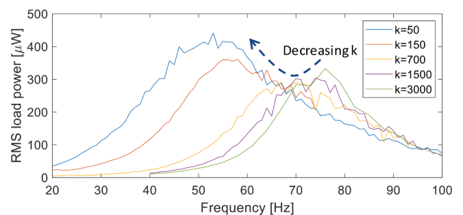
Fig. 10. EMEH RMS load power spectrum for different values of the J-A parameter k. The remaining J-A parameter values are constant (see Table 4: Right). The models use a spring constant of 100 N/mm and spring offset of 2.11 mm. The remanence of the magnet in each of these simulations is 1.4 T.
