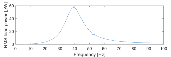
Fig. 14. Frequency response using parameterization tuned to 40 Hz.
