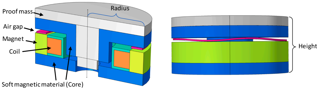
Fig. 1. Electromagnetic energy harvester concept design with ideal spring placement. Schematic of geometry and constituents.
