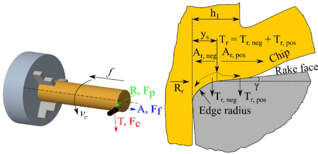
Fig. 12 Definition of main directions and force directions in a general turning process and a section of an engaged tool with the forces that act on the rake face of a cutting tool. Modified after Ståhl [17] and Schultheiss [44]
