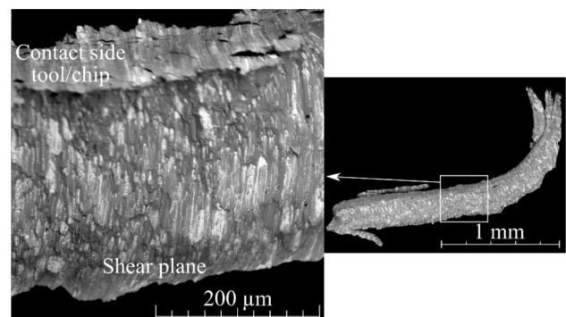
Fig. 20 Backscatter image of the shear plane on a CuZn38Pb3 chip. Bright areas are lead
