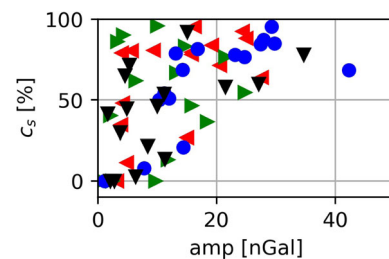
Fig. 8 Relationship between signal amplitude and captured signal fraction for ^3M_1 (blue circles), ^3N_2 (green triangle), ^3L_2 (red triangle) and ^3M_3 (black triangle). Negative agreement c < 0 is displayed as 0%
