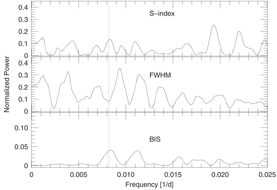
Figure 6. GLS periodogram of the activity indicators after removal of the dominant signal in each (Table 5). The vertical dashed line is the frequency of the 125 day period seen in the RV data.
