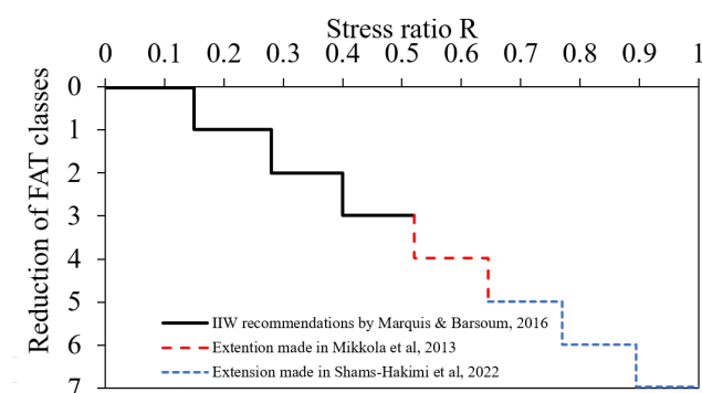
Figure 1. Proposed reduction in fatigue strength class depending on the stress ratio.
