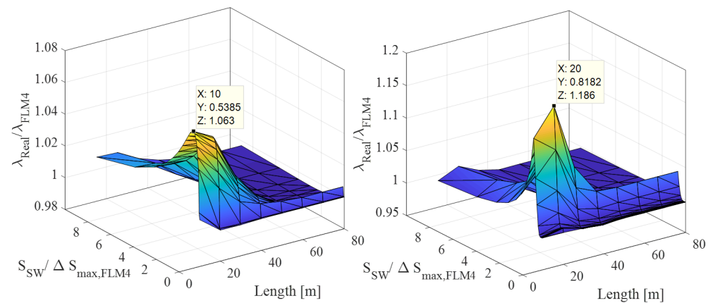
Figure 12. The ratio of \lambda_{\text{HFMI}} for original real traffic in Sweden and \lambda_{\text{HFMI}} for FLM4 (long-distance traffic) calculated for mid-span section (to the left) and mid-support section (to the right).
