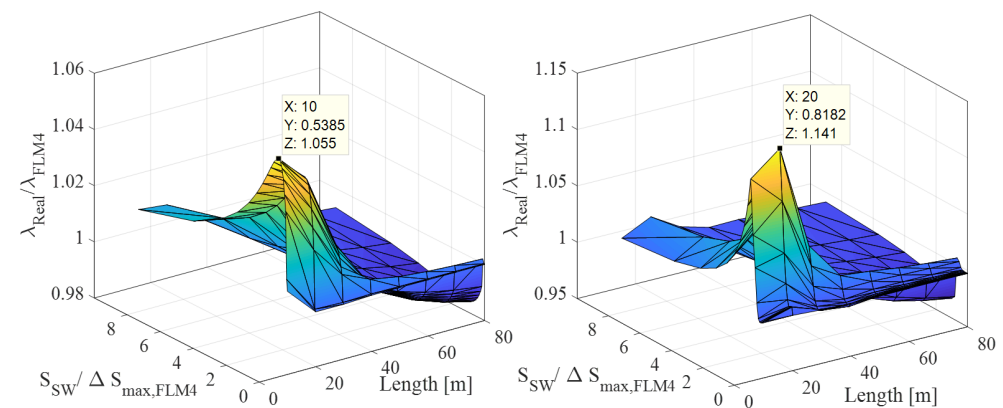
Figure 13. The ratio of \lambda_{\text{HFMI}} for original real traffic in Sweden and \lambda_{\text{HFMI}} for FLM4 (medium-distance traffic) calculated for mid-span section (to the left) and mid-support section (to the right).
