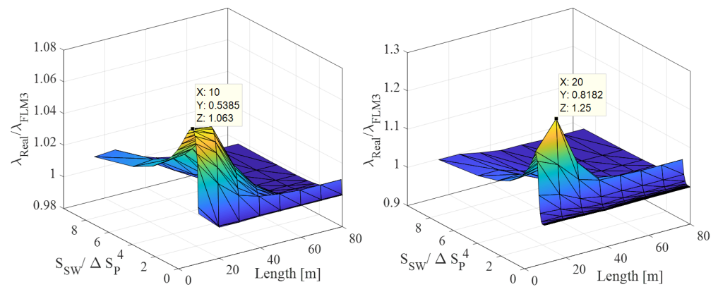
Figure 11. The ratio of \lambda_{\text{HFMI}} for original real traffic in Sweden and \lambda_{\text{HFMI}} for FLM3 calculated for the mid-span section (to the left) and mid-support section (to the right).
