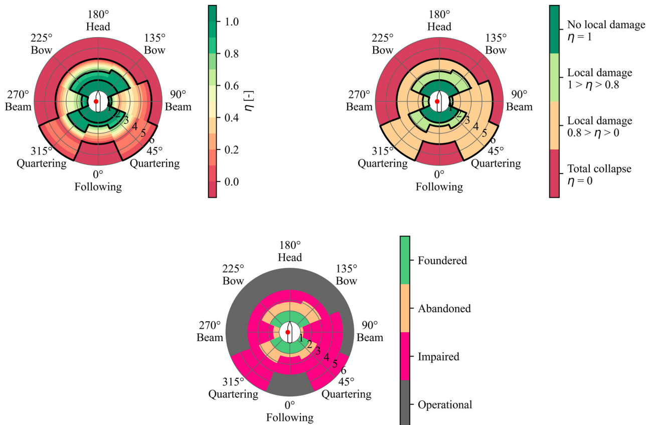
Figure 11. Polar plots of (upper left) structural adequacy, (upper right) structural state and (lower) vessel condition with respect to structural limit states for different wave-encountering directions and significant wave heights (This figure is available in colour online.)
