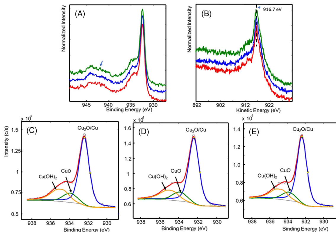
FIGURE 4 X-ray photoelectron spectroscopy (XPS) high-energy resolution spectrum of (A) \text{Cu}2p_{3/2} core level and (B) \text{Cu } L_3M_{45}M_{45} Auger peak recorded from the surface of copper powders. Curve fitting of \text{Cu}2p_{3/2} core level is also shown for powders with distribution of particle sizes (C) D_{90} < 16 , (D) 22, and (E) 31 \mu\text{m}
