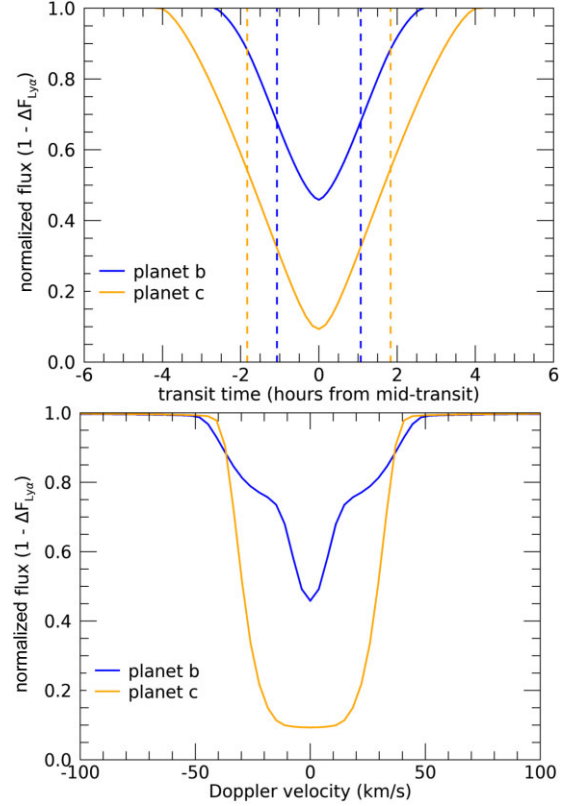
Figure 13. Top: Ly \alpha light curves for planet HD 73583 b (blue) and HD 73583 c (orange). The dashed lines mark the duration of the geometric transit. Bottom: Normalized absorption profile at mid-transit for planet HD 73583 b (blue) and HD 73583 c (orange).
