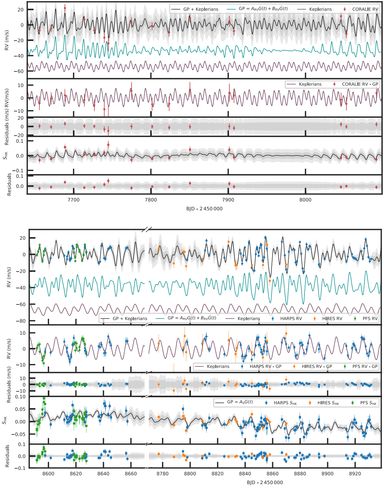
Figure 7. RV and S_{HK} time-series after been corrected by inferred offsets. Each plot shows (from top to bottom): RV data together with full, stellar, and planetary signal inferred models; RV data with stellar signal model subtracted; RV residuals; S_{HK} data together with inferred stellar model, and S_{HK} residuals. The upper plot shows CORALIE (red) observations. The bottom plot displays HARPS (blue), HIRES (orange), and PFS (green) data. Measurements are shown with filled symbols with error bars with a semitransparent error bar extension accounting for the inferred jitter. The solid (black) lines show the inferred full model coming from our multi-GP, light grey shaded areas showing the 1 \sigma and 2 \sigma credible intervals of the corresponding GP model. For the RV time-series we also show the inferred stellar (cyan line) and planetary (dark purple line) recovered signals with an offset for better clarity. We note that in the bottom plot there is a gap between 8670 and 8770 BJD - 2450000 where there were no measurements.
