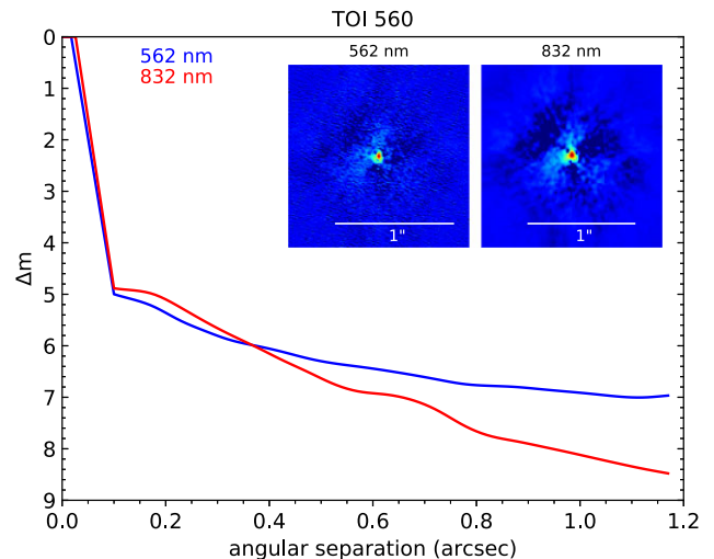
Figure 2. Contrast curves showing the 5\sigma detection sensitivity obtained using Zorro on Gemini with the filters centred on 562 nm (blue line) and 832 nm (red line). No bright companions are detected within 1.2 arcsec to HD 73583.
