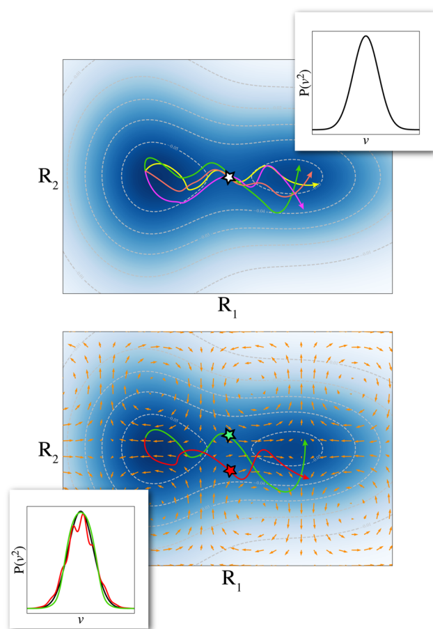
FIG. 2. Illustrative sketch of different trajectories evolving on a double-well potential energy surface (blue sinks with gray isosurfaces) in canonical equilibrium (top) vs stationary non-equilibrium dynamics (bottom). Units are chosen arbitrarily. Note that the probability density P(v^2) of each velocity degree of freedom is normally distributed in canonical equilibrium, where the temperature is related to its variance. In contrast, the emergence of (time-dependent) non-conservative forces (orange arrows) modifies the physical properties fundamentally when coupled to a thermal bath. In that case, the stationary probability densities can deviate considerably from the Boltzmann solution. Moreover, one cannot necessarily identify relevant transition states (green and red star) from saddle points of the potential energy surface (white star). All of which effects could be relevant for the theoretical description of polaritonic reaction rates under vibrational strong coupling.
