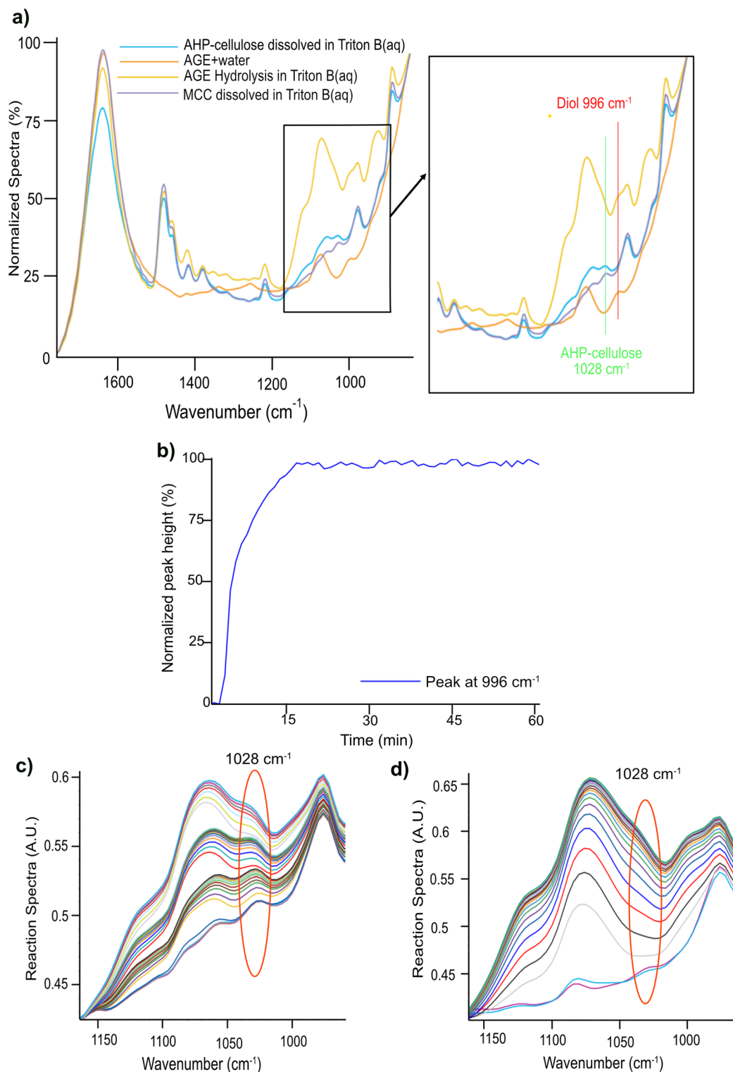
Fig. 5 (a) Spectra comparison for peak assignment (b) Peak at 996\text{ cm}^{-1} in AGE hydrolysis in absence of MCC (in Triton B) (c) MCC etherification by AGE addition in aliquots in Triton B for 4 h (d) AGE hydrolysis in Triton B for 4 h.
