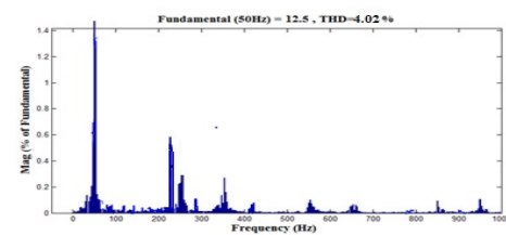
Figure 15. THD analysis of line current at load side-SM controller
