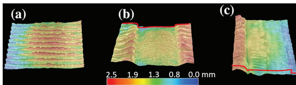
Figure 19. The 3D profiles of the extrudates obtained by a) slit die with H = 3 mm, W = 10 mm at \dot{\gamma}_{app}^{H=3mm} = 7 \text{ s}^{-1} , b) slit-die-simple-profile with H = 3 mm, H = 2 mm, W = 10 mm, at \dot{\gamma}_{app}^{H=2mm} = 7 \text{ s}^{-1} , \dot{\gamma}_{app}^{H=3mm} = 7.7 \text{ s}^{-1} , and c) slit-die-scalar-profile with H = 3 mm, H = 2 mm, H = 1.5 mm and W = 10 mm, at \dot{\gamma}_{app}^{H=1.5mm} = 37.3 \text{ s}^{-1} , \dot{\gamma}_{app}^{H=2mm} = 7 \text{ s}^{-1} , and \dot{\gamma}_{app}^{H=3mm} = 9.3 \text{ s}^{-1} , see Figures 2, 14, and 17 for the dies. All the dies have a length of L = 30 mm and the profile for the b–c) is existing at L_{profile} = 3 mm before the die exit. The extrudate was obtained at T = 100 °C.
