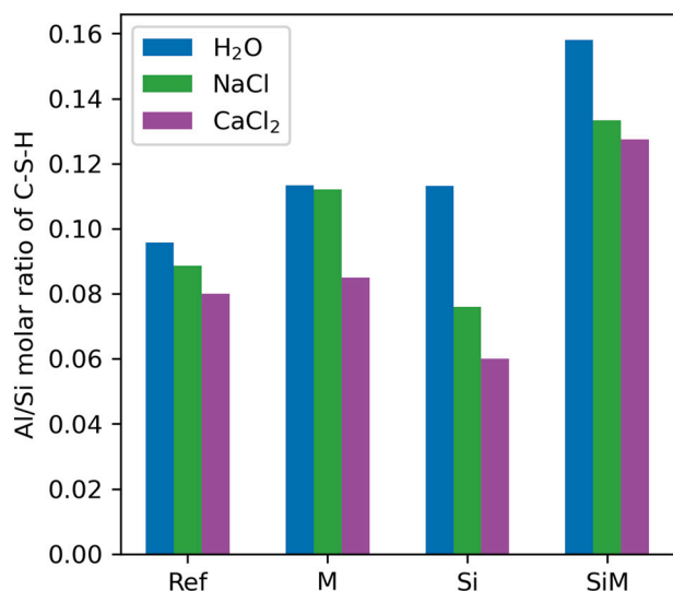
Fig. 8. Al/Si molar ratio of the C(-A)-S-H based on the deconvoluted ^{29}\text{Si} NMR spectra from the Ref, M, Si and SiM binder's pastes exposed to water ( \text{H}_2\text{O} ), NaCl or \text{CaCl}_2 solutions with a 2 mol/L chloride concentration.
