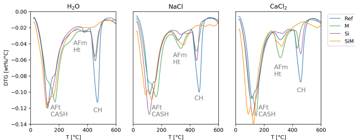
Fig. 2. DTG curves in the 50 °C to 600 °C range for the Ref, M, Si and SiM binder's pastes exposed to water (H 2 O), or NaCl or CaCl 2 solutions with a 2 mol/L chloride concentration. The mass-loss peaks typically associated with Aft, C(-A)-S-H, AFm, hydrotalcite (Ht) and portlandite (CH) are marked.
