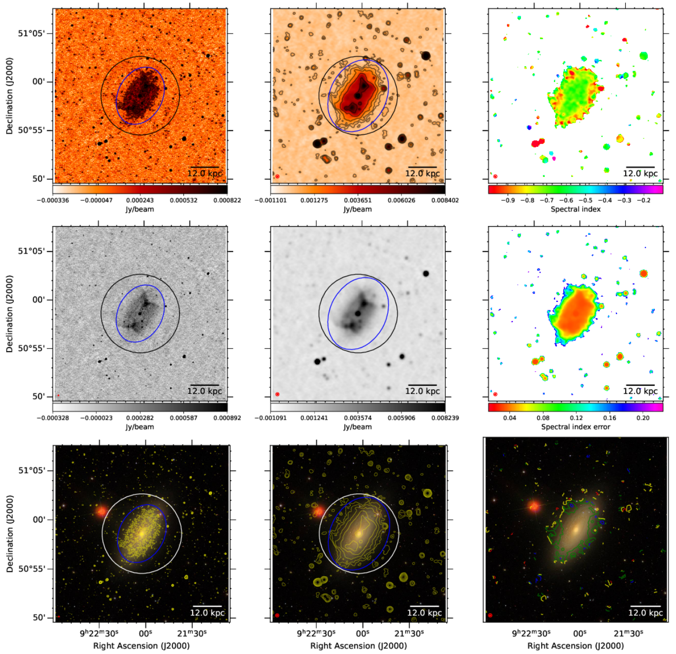
Fig. B.8. NGC 2841. The first row shows from left to right the 144-MHz maps at 6 and 20 arcsec resolution, respectively, and the radio spectral index map between 144 and 1365 MHz at 20 arcsec resolution. Contours start at 3\sigma with increments of a power of two. The black circle shows the optical D_{25} diameter and the blue ellipses show the 3\sigma contour extent used to integrate the flux density. The second row shows again the 6- and 20-arcsec images without contours and the radio spectral index error. The third row shows the 6- and 20-arcsec contours overlaid on an rgb SDSS image as well as contours of the radio spectral index. The filled circle shows the synthesised beam. A scale bar shows the projected size at the distance of the galaxy.
