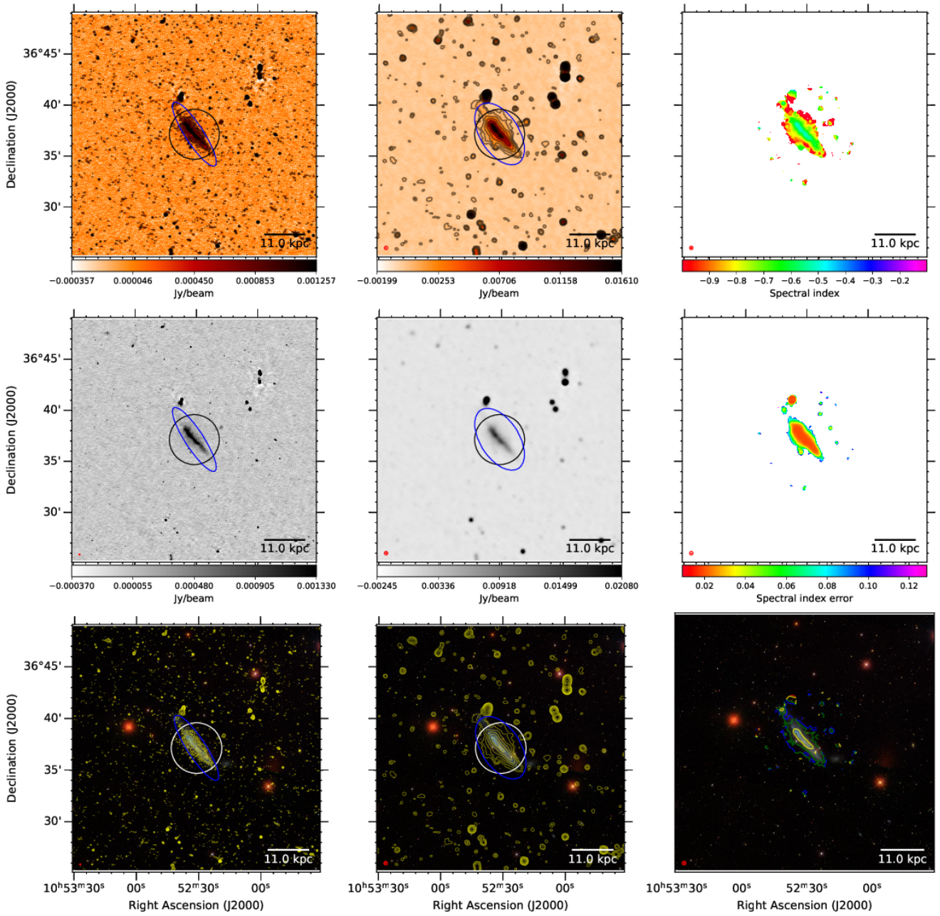
Fig. B.18. NGC 3432. The first row shows from left to right the 144-MHz maps at 6 and 20 arcsec resolution, respectively, and the radio spectral index map between 144 and 6000 MHz at 20 arcsec resolution. Contours start at 3\sigma with increments of a power of two. The black circle shows the optical D_{25} diameter and the blue ellipses show the 3\sigma contour extent used to integrate the flux density. The second row shows again the 6- and 20-arcsec images without contours and the radio spectral index error. The third row shows the 6- and 20-arcsec contours overlaid on an rgb SDSS image as well as contours of the radio spectral index. The filled circle shows the synthesised beam. A scale bar shows the projected size at the distance of the galaxy.
