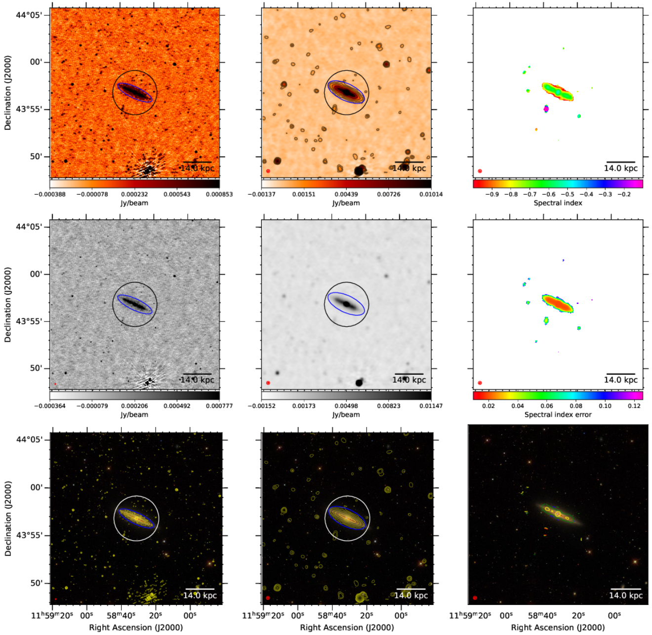
Fig. B.23. NGC 4013. The first row shows from left to right the 144-MHz maps at 6 and 20 arcsec resolution, respectively, and the radio spectral index map between 144 and 6000 MHz at 20 arcsec resolution. Contours start at 3\sigma with increments of a power of two. The black circle shows the optical D_{25} diameter and the blue ellipses show the 3\sigma contour extent used to integrate the flux density. The second row shows again the 6- and 20-arcsec images without contours and the radio spectral index error. The third row shows the 6- and 20-arcsec contours overlaid on an rgb SDSS image as well as contours of the radio spectral index. The filled circle shows the synthesised beam. A scale bar shows the projected size at the distance of the galaxy.
