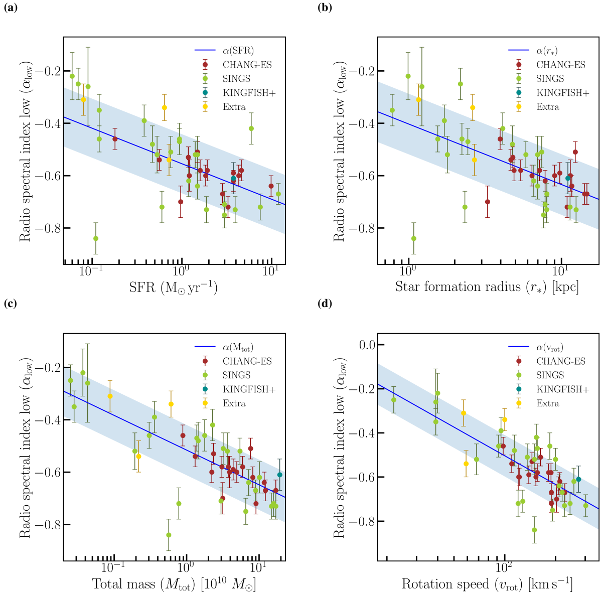
Fig. 5. Radio spectral index as a function of several fundamental galaxy parameters. Panel a: dependence on SFR as calculated from the TIR luminosity; (b): dependence of the star formation radius, which is derived from the extent of the 3\sigma contours in the 20 arcsec LoTSS images; (c): dependence on the total mass calculated; (d): dependence on the rotation speed. In all panels, the blue line is the best-fitting relation and the shaded areas show 1\sigma confidence intervals. The colours of the data points in panel b indicate the rotation velocity, in the other panels the colours indicate the different subsamples.
