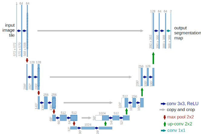
Fig. 6. U-Net architecture.
