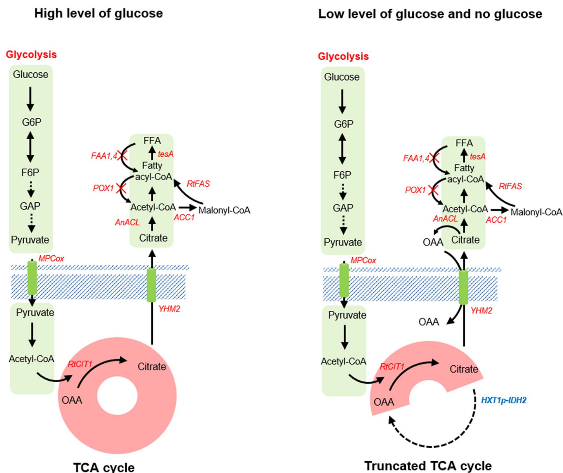
Extended Data Fig. 3 | The genetic modifications in the strains Y&Z032. The IDH2 (Subunit 2 of mitochondrial NAD(+) -dependent isocitrate dehydrogenase) gene in Y&Z032 is expressed by the HXT1 promoter, which is induced at high and suppressed at low glucose concentrations. Other modifications were also shown in Figure.
