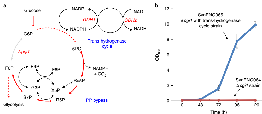
Fig. 1 | Detoxification of extra NADPH by the trans-hydrogenase cycle.
