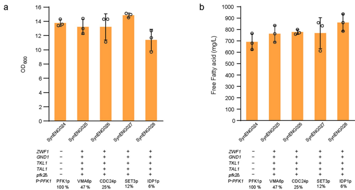
Extended Data Fig. 4 | Synthetic energy system support FFAs production. Increased decarboxylation benefit FFAs production. Fine-tune of glycolysis was achieved by down regulation of phosphofructokinase PFK1 and the deletion of PFK2. The native PFK1 promoter (100%) was replaced by weaker promoter of VMA6p (47%), CDC24 (25%), SET3 (12%), IDP1 (6%), separately. The cell growth and fatty acid level were shown in figure a and figure b . Statistical analysis was
