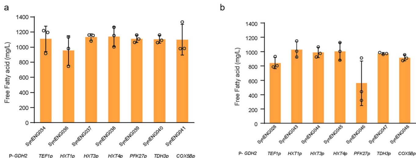
Extended Data Fig. 6 | Dynamic regulation of the transhydrogenase cycle. a , Dynamic regulation of the transhydrogenase cycle have no effect on FFAs production with high NADPH supply. Dynamic regulation of the transhydrogenase cycle was achieved by fine-tuning of GDH2 expression. Carbon source dependent promoters, such as HXT1 , HXT3 , HXT4 , PFK27 and COX5B , were used. These promoters were induced by high levels of glucose and repressed by low levels of glucose. TDH3 promoter was used as a second control. The background strain SynENG034 have high level of NADPH supply as shown in Fig. 4d. b , Dynamic regulation of the transhydrogenase cycle have no effect on FFAs production with low NADPH supply. Dynamic regulation of the transhydrogenase cycle was achieved by fine-tuning of GDH2 expression.
