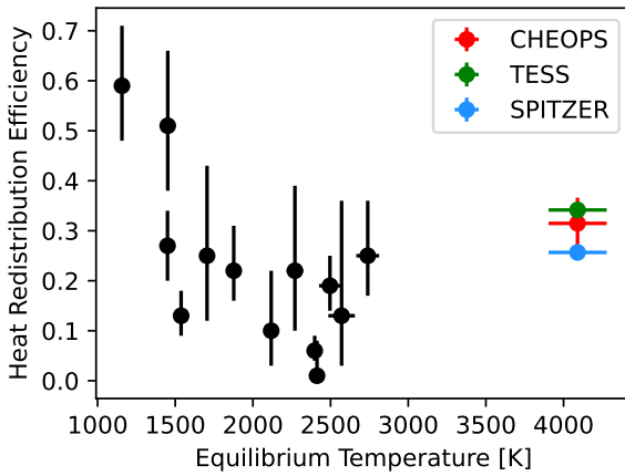
Fig. 9. Heat redistribution efficiency of hot Jupiters plotted against their equilibrium temperatures. The coloured points show the KELT-9b efficiency, \varepsilon , derived in this study.
