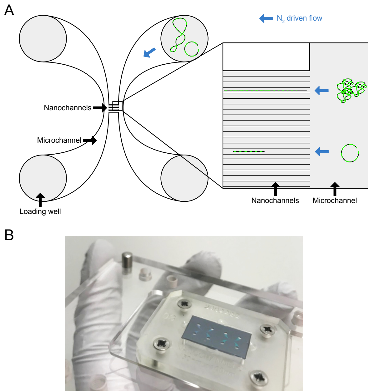
FIGURE 13: IN A, THERE IS AN OVERVIEW OF A NANOFLUIDIC CHIP WITH ITS MAIN FEATURES FOR STRETCHING OF DNA (NOT DRAWN TO SCALE). THE MAIN FEATURES ARE THE NANOCHANNELS SPANNING THE TWO MICROCHANNELS, THAT IN TURN ARE CONNECTING TWO AND TWO OF THE LOADING WELLS THAT CAN BE PRESSURED WITH NITROGEN-DRIVEN FLOW. IN B, THERE IS AN IMAGE OF A NANOFLUIDIC CHIP MOUNTED ON A HOLDER.
