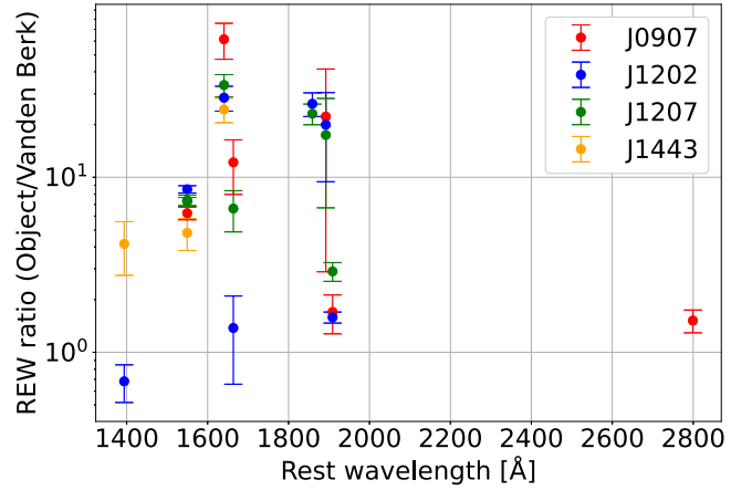
Figure 9. REW ratio vs. rest-frame wavelength. REW ratios are defined as REWs of objects over REWs from the composite spectrum of SDSS type 1 quasar measured by Vanden Berk et al. (2001). The red, blue, green, and orange plots show the REW ratios of J0907, J1202, J1207, and J1443, respectively.
