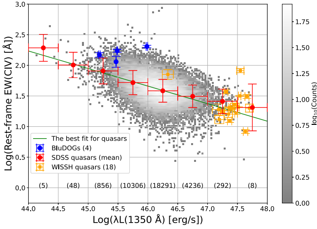
Figure 10. REW of the C IV vs. the monochromatic luminosity at 1350 Å. Blue and orange dots represent the four BluDOGs and WISSH quasars (Vietri et al. 2018). The gray 2D histogram represents the number density of the SDSS quasars (Shen et al. 2011). The green line represents the linear fit to the distribution of the SDSS quasars. The red plots show the mean and standard deviation in luminosity bins with 0.5 dex width. The numbers of SDSS quasars in the individual bins are shown at the bottom of the panel.
