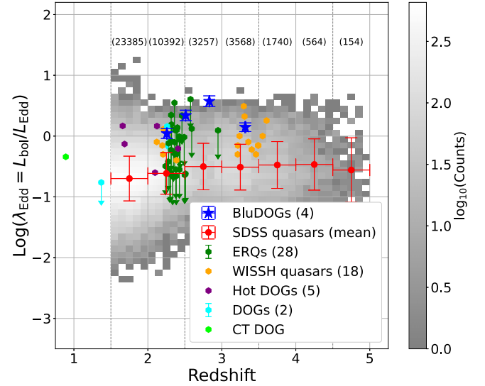
Figure 12. Diagram of the redshift vs. the Eddington ratio. The filled-blue stars and hexagons are the same as in Figure 11. The gray 2D histogram represents the number density of SDSS quasars (Shen et al. 2011). The red plots show the mean and standard deviation of \lambda_{\text{Edd}} in redshift bins with a width of \Delta z = 0.5 . The numbers shown at the upper part denote the numbers of SDSS quasars in the redshift bins.
