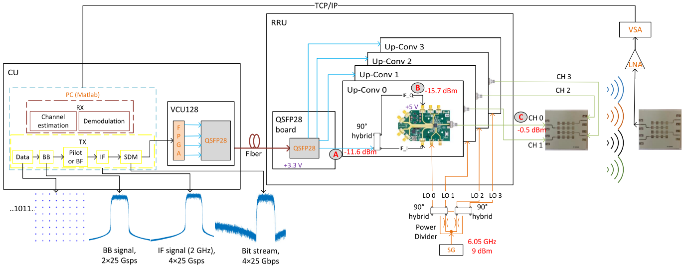
Fig. 1. The link architecture of the demonstration. At CU, the PC and FPGA generate the SDM signal to the optical fiber. The QSP28 connected RRU has four parallel upconversions to radiate signal through a linear array patch antenna.
