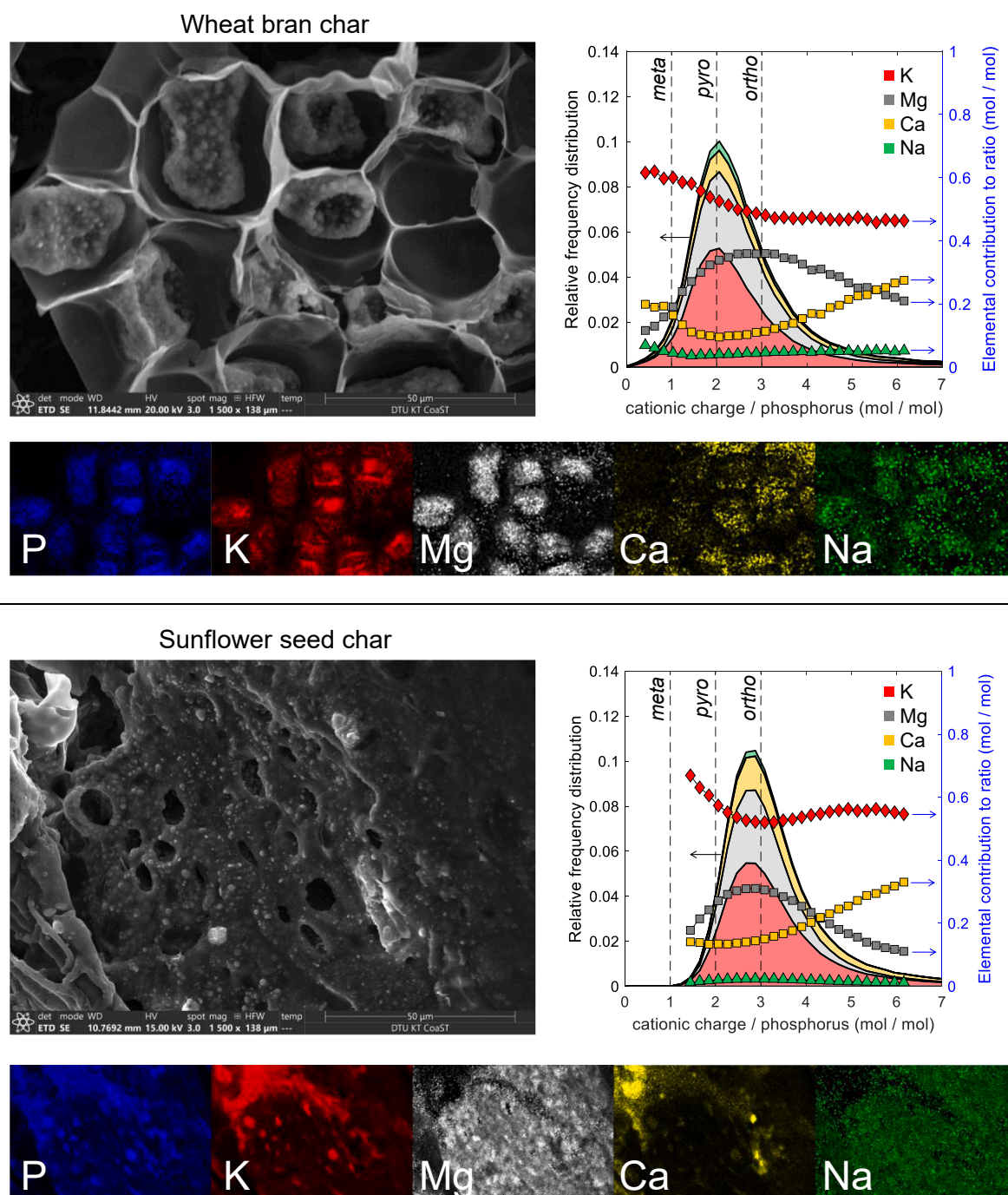
Fig. 2. SEM images of wheat bran char (upper) and sunflower seed char (lower) produced in N_2 at 800^\circ C using a holding time of 10 min, with EDS mapping showing the major ash-forming elements (excluding carbon and oxygen). The intensity of the EDS maps are scaled individually to show the location of each element and does not represent concentration relative to other elements. Note that almost no sodium was detected for the sunflower seed char, but it has been included here for consistency. The molar ratio of cationic charge/phosphorus atom was calculated for each of the pixels in the EDS-maps and are shown in graphs as relative frequency distributions scaled proportionally using the content of phosphorus in each pixel. Symbols (right axis) represent the contribution of each cation to the cationic charge/phosphorus atom ratio. The cationic charge/phosphorus atom ratio in meta-, pyro-, and orthophosphates are shown using vertical dashed lines.
