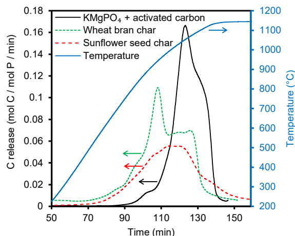
Fig. 12. Carbon release rate, calculated using CO + \text{CO}_2 concentration in flue-gas and scaled using the molar amount of phosphorus in the original sample, (left axis) and temperature (right axis) when heating wheat bran char, sunflower seed char, or \text{KMgPO}_4 mixed with activated carbon, from 25 to 1135\text{ }^\circ\text{C} in 3 L/min N_2 .
