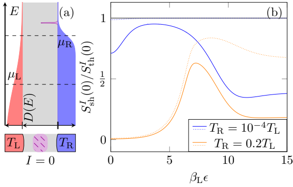
FIG. 3. (a) Zero-charge-current condition for the Lorentzian transmission D(E) from Eq. (23) (depicted in purple), with fixed \beta_L \Gamma = 10^{-2} and D_0 = 0.5 . (b) Charge noise ratio S_{sh}^I(0)/S_{th}^I(0) for the Lorentzian transmission as a function of the resonance peak position \epsilon and for two different temperatures of the cold reservoir. Dotted lines correspond to the bound in Eq. (22). The solid, grey line corresponds to the bound in Eq. (18).
