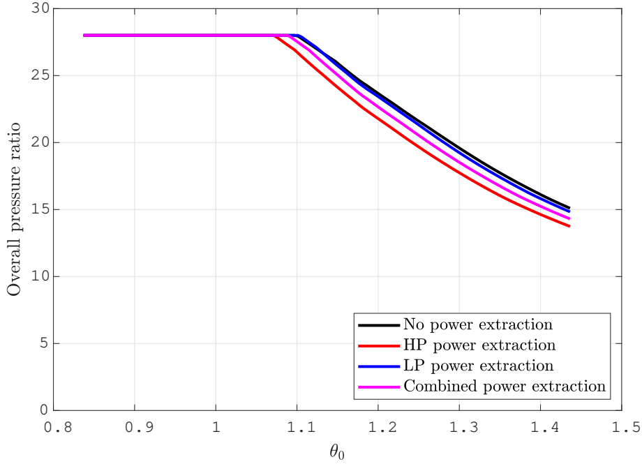
Figure 4.4: OPR versus \theta_0 , altitude 9 km at military power.
