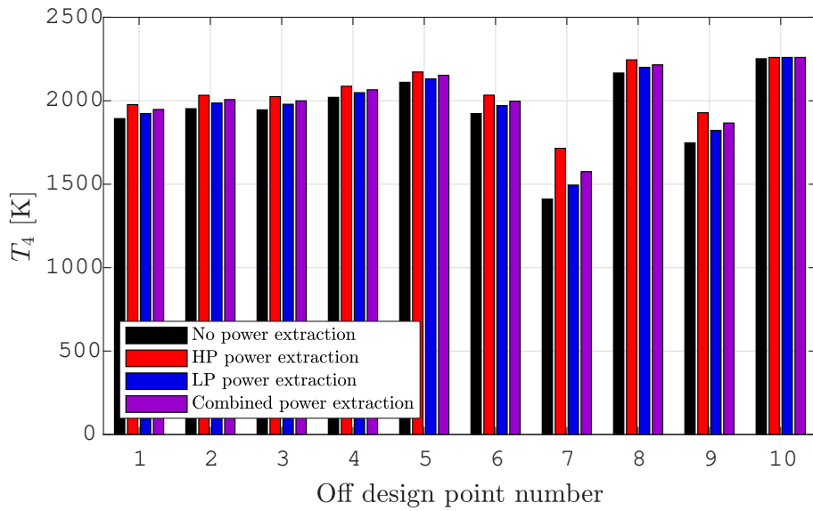
Figure 4.2: Turbine inlet gas temperature.
