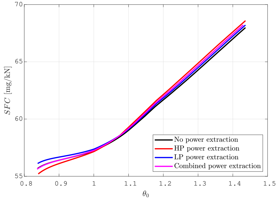
Figure 4.11: SFC versus \theta_0 , altitude 9 km at MAX power.
