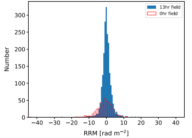
Figure 11. Top: Histogram of the RM values for the 2461 polarized sources in both the 13 h field and 0 h field of the LoTSS-DR2 area. The spread represents the dominant contribution of the Galactic RM (GRM). The gap near 0 \text{ rad m}^{-2} is due to the exclusion of sources contaminated by the instrumental polarization present in LOFAR data. Bottom: Histogram of the residual rotation measure (RRM) after subtraction of the model GRM, for the 13 h field (blue solid) and for the 0 h field (red open).
