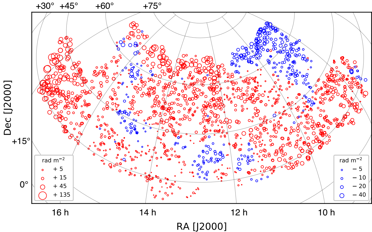
Figure 3. Sky distribution of the polarized sources across the LoTSS-DR2 13 h field, in equatorial coordinates and with an orthographic projection. The red/blue coloured circles correspond to positive/negative RM values, and the size of the circles are proportional to the magnitude of the RM (as quantified in the figure legends). There are 2039 sources in the 13 h field, which corresponds to an areal number density of 0.48 deg -2 .
