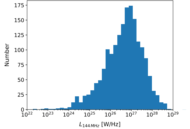
Figure 20. Histogram of the radio luminosity at 144 MHz, in \text{W Hz}^{-1} , for all sources with a redshift estimate (either spectroscopic or photometric). The median 144 MHz luminosity is \sim 5 \times 10^{26} \text{ W Hz}^{-1} .
