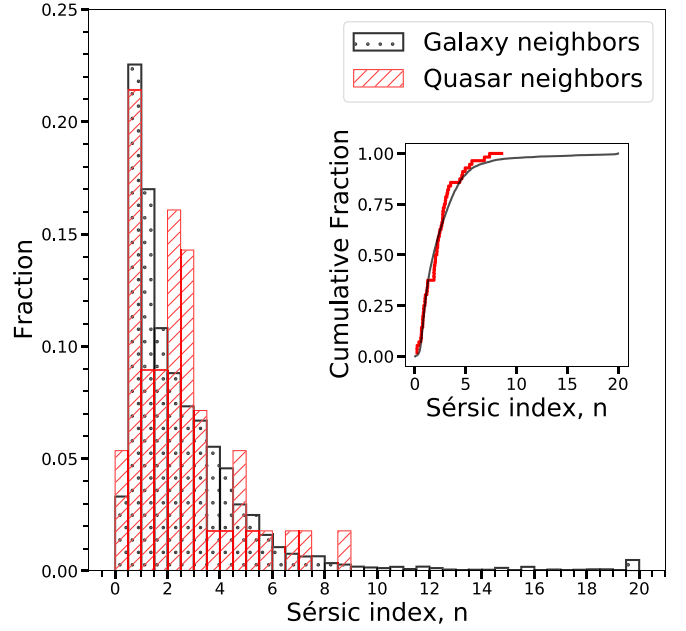
Figure 11. Sérsic index (quasar neighbors in red hatched bars, comparison galaxy neighbors in black dotted bars). The inset shows the eCDF, quasar neighbors in red solid line, and comparison galaxy neighbors in black. Median error for Sérsic index values from GAMA is \sim 0.14 both for quasar neighbors and for comparison galaxy neighbors.
