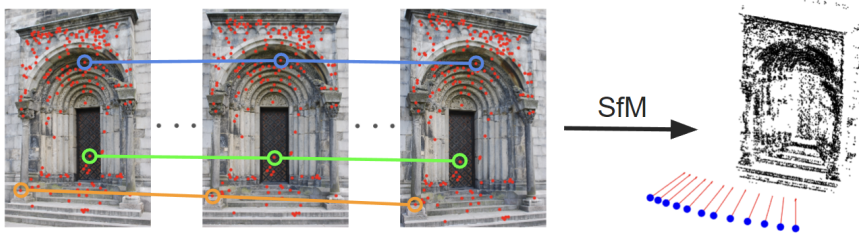
Figure 1.1: Representation of the inputs and outputs of a Structure-from-Motion (SfM) algorithm. (Left) Multiple images are captured from different viewpoints of a certain object or scene, in which keypoints (in red) are detected and matched along the images (some of the matches are represented in blue, green and yellow). (Right) These matches, or correspondences, are then fed as input to a Structure-from-Motion algorithm, which ultimately estimates the 3D coordinates of the detected keypoints (in black), along with the camera calibrations position (in blue), rotation (red arrows) and internal calibration.
