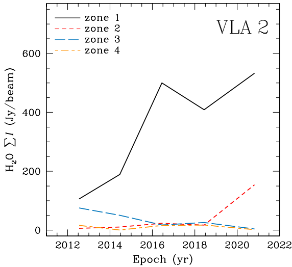
Fig. 10. Comparison of the total \text{H}_2\text{O} maser intensity in the four zones of VLA 2 (see Fig. 4) measured in epochs 2012.54 (VLBA; S14 ), 2014.46 (EVN), 2016.45 (EVN), 2018.44 (EVN), and 2020.82 (EVN).
