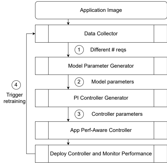
Figure 2: DDPC Pipeline
