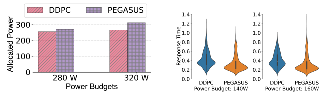
(a) The power allocation of both Pegasus and DDPC under the two different caps. (b) Violin plots of the distribution of response times under the two different caps.
