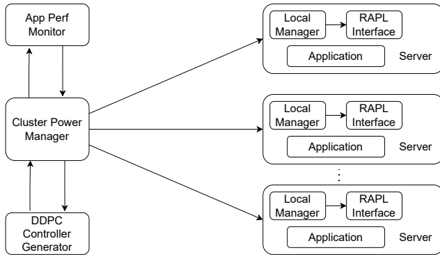
Figure 1: The DDPC architecture
