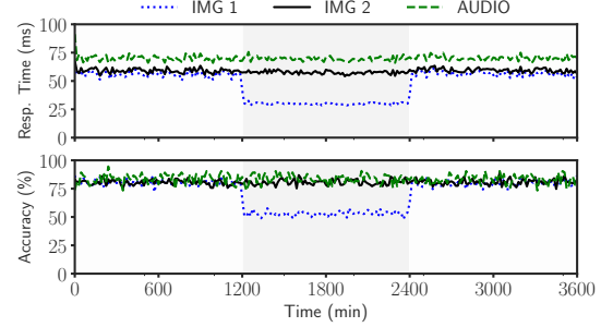
Figure 14: Non-Cooperative local MAX-MIN adaptation.
