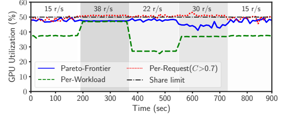
Figure 13: The effect of limiting resources to an individual application across different request rates.
