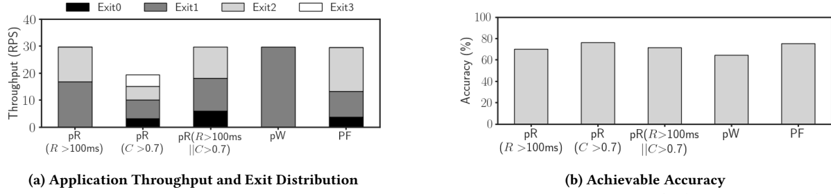
Figure 7: The application throughput, exit distribution, and accuracy for per-request (pR), per-workload (pW), and Pareto-frontier (PF) adaptation policies. D len runs ResNet50 and has a workload of 30 requests/second.
