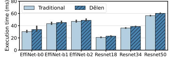
Figure 16: The overhead of Delen's conditional execution framework compared to traditional (single exit) approach.
