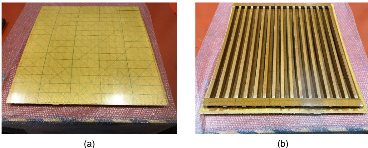
Figure 6 – 700 x 700 mm rib-stiffened monolithic composite fuselage-integrated radome. (a) top and (b) bottom views
