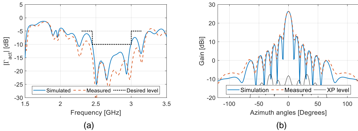
Figure 5 – The performance of the 16×16 elements antenna array demonstrator when the main beam is at broadside. Measurement and simulation results of (a) total active reflection coefficients and (b) radiation patterns at 2.7 GHz.
