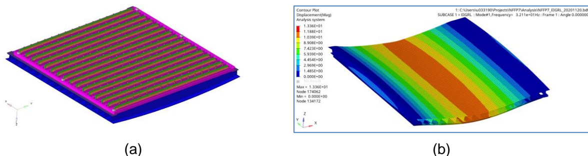
Figure 7 – FE-model and the mode shape. (a) FEM simulation model and (b) Lowest order eigenmode
