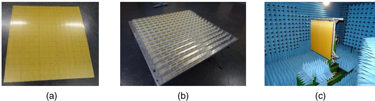
Figure 4 – Pictures of the 16×16 elements antenna array demonstrator. Antenna array (a) with radome, (b) without radome and (c) in the measurement chamber.
