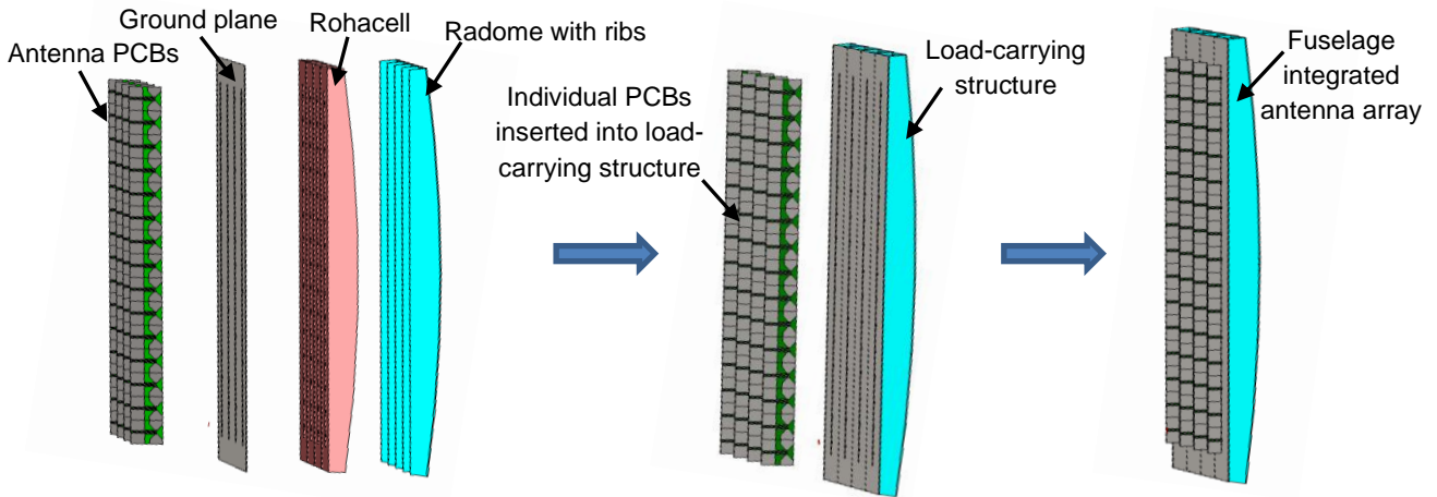
Figure 3 – Fuselage integrated antenna array and its assembly
