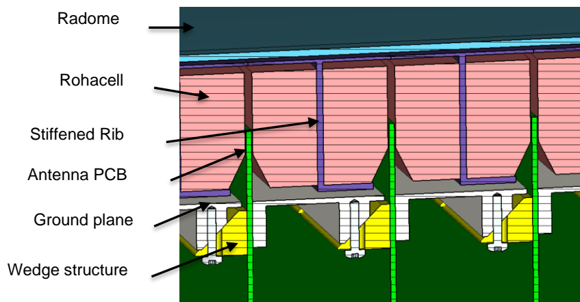
Figure 2 – Cross-section view of the antenna array
