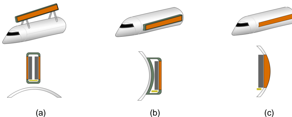
Figure 1 – Antenna configurations on the airborne early warning platform. (a) dorsal mounted, (b) side-mounted and (c) fuselage integrated.
