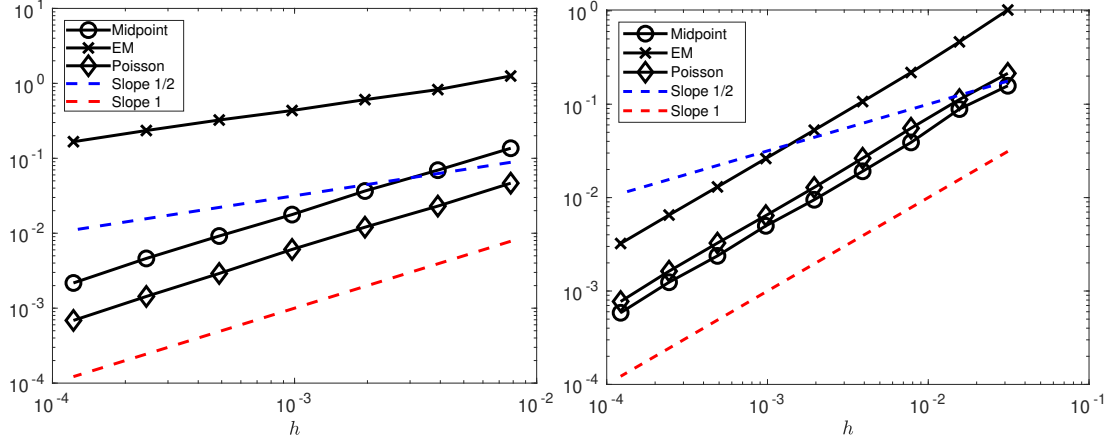
FIGURE 2. Stochastic Maxwell–Bloch system with a single Wiener process: Strong errors of the Euler–Maruyama scheme ( \times ), the midpoint scheme ( \circ ), and the explicit stochastic Poisson integrator ( \diamond ). Left: (\sigma_1, \sigma_3) = (1, 0) . Right: (\sigma_1, \sigma_3) = (0, 1) .
