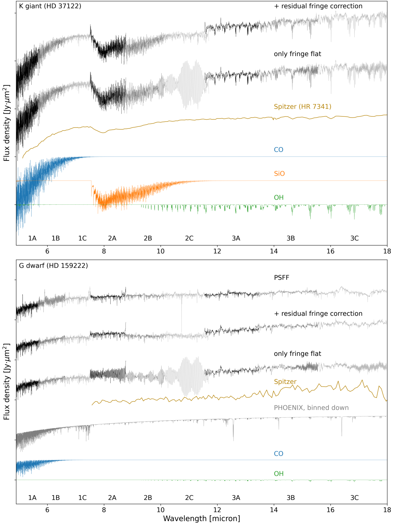
Fig. 10. Spectra for HD 37122 (top) and HD 159222 (bottom), after applying only the extended fringe flat, extended fringe flat and residual fringe correction, or the point source specific correction labelled “PSFF”). The y -axis is in Rayleigh-Jeans units, resulting in a flat tail of the stellar spectrum. The sub-bands (A, B, C) are indicated by increasingly light colours; blue, orange, and green are the model CO, SiO, and OH spectra, respectively. The Spitzer spectra are taken from Sloan et al. (2015, top panel) and the CASSIS database (Lebouteiller et al. 2011; bottom panel).
