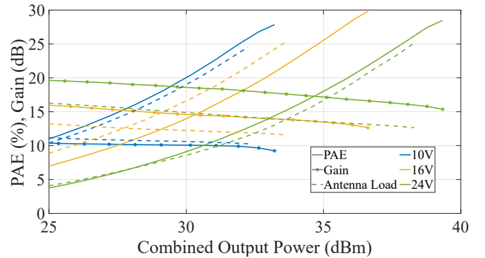
Fig. 4. Measured CW efficiency and gain for the array at 6.5 GHz with the four PAs loaded with 50\ \Omega loads (solid) and with antenna elements (dotted). The PAE curves for different supply voltages are measured statically and averaged across the 4 PAs.
