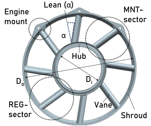
Fig. 4. Map of some of the key components and design variables of the TRS.
