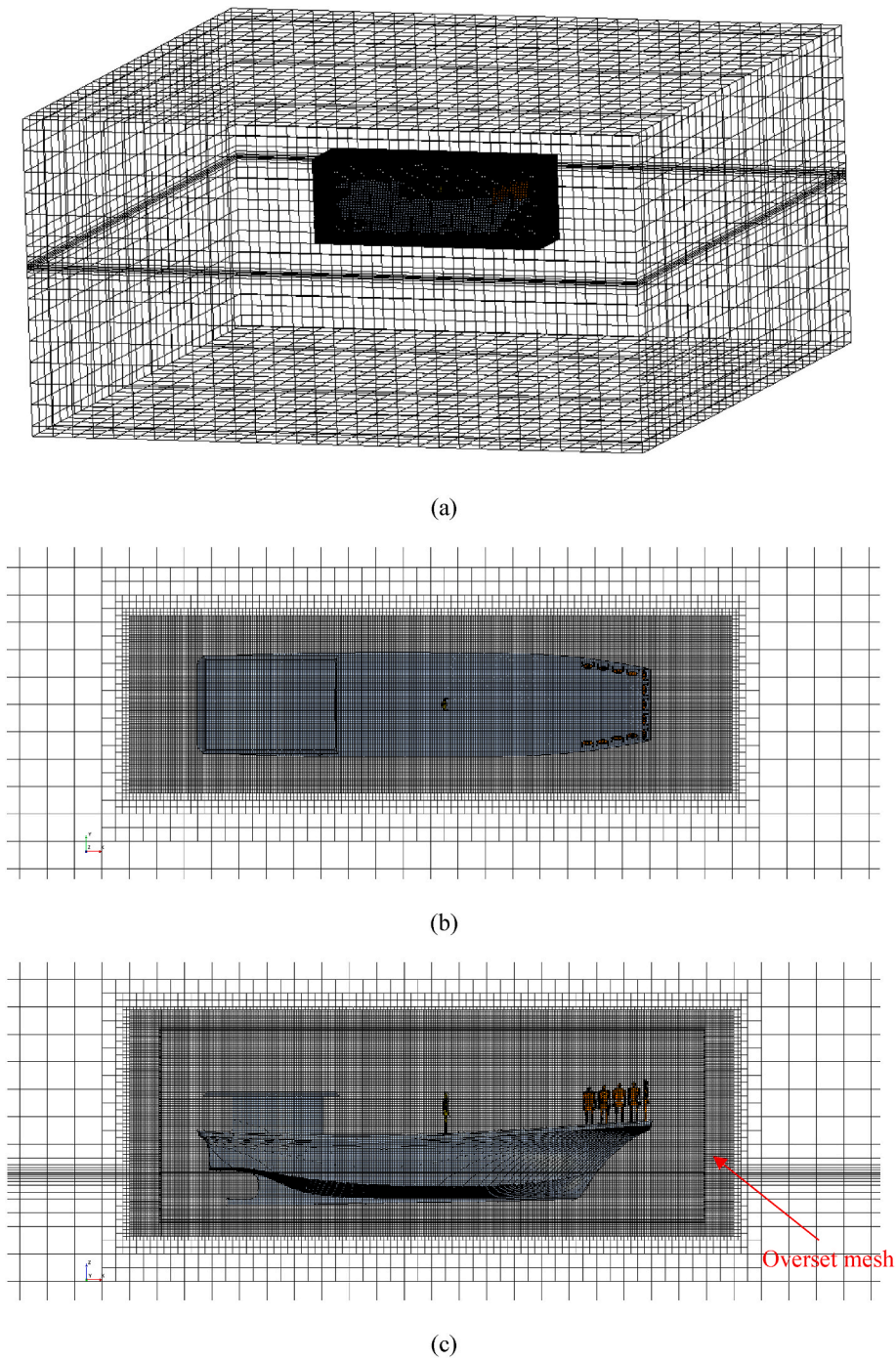
Fig. 7. Discretised computational domain with local refinements applied to overset and free surface regions: (a) Whole domain, (b) Plan view close-up, (c) Profile view close-up.
