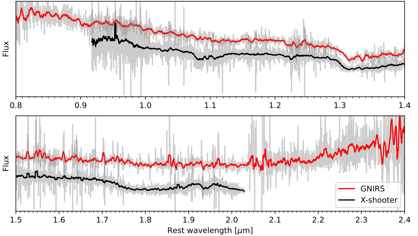
Fig. 5. NIR spectra for SN 2019wxt taken on 19 Dec 2019. Grey lines show original spectra, colour lines have been smoothed with a Savitzky-Golay filter with window length 50 Å. We do not include the GTC/EMIR spectrum which has low S/N.
