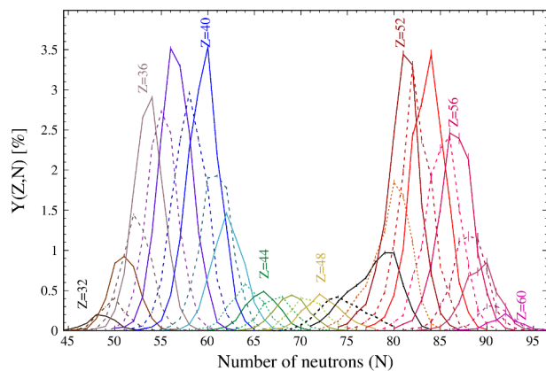
Figure 8. Experimental isotopic yields, with their uncertainties, measured for ^{236}\text{U}(\gamma,\text{f}) with the \text{R}^3\text{B}/\text{SOFIA} setup. Isotopic yields for Z = 49 and Z = 50 are represented in black dashed and full lines, respectively.
