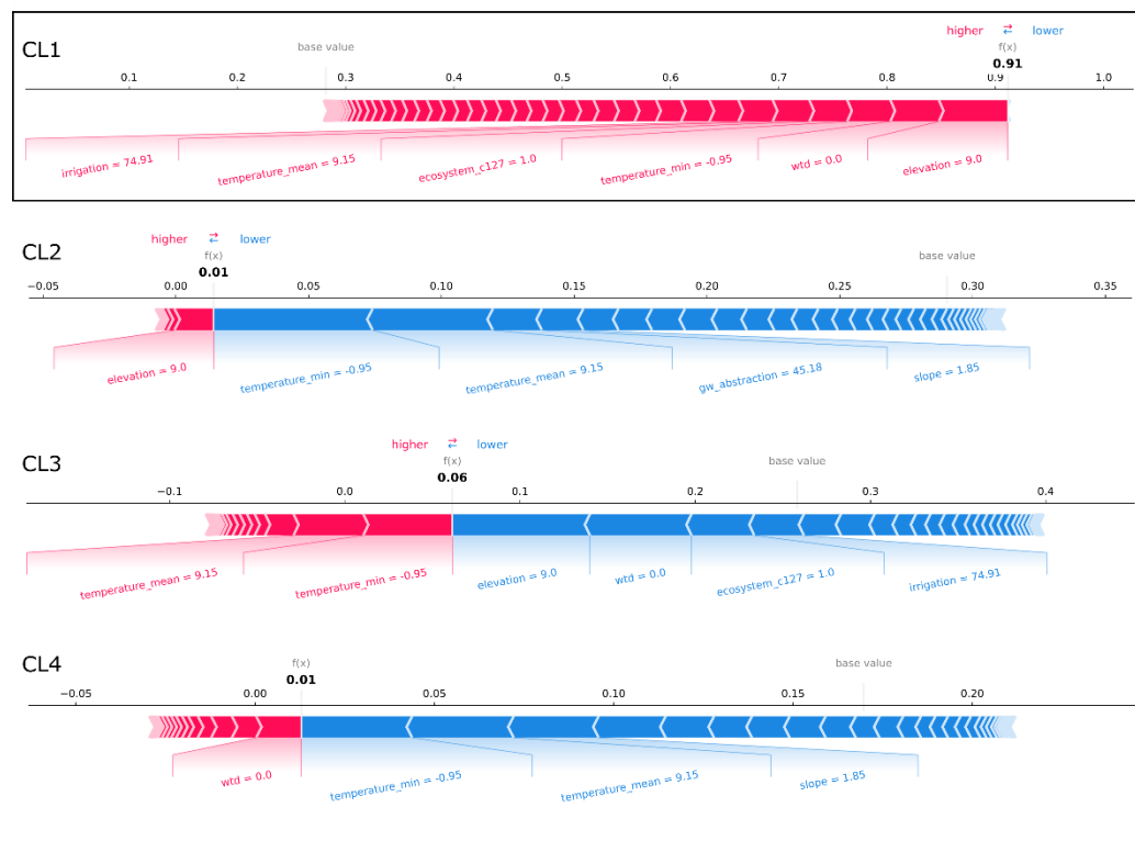
Figure E4 SHAP force plots explaining the correct prediction of the CL1 exemplary well site from the case study region in northern Germany (Fig. 5a) (from top to bottom: CL1, CL2, CL3, and CL4). At this well site, the probability that CL1 is predicted is the largest in the case study (test dataset). The average scores of all classifications made by the Random Forest model for the training dataset are 0.28, 0.29, 0.26, and 0.17 respectively (base values). The model's probability scores for predicting the clusters at the exemplary well site (bold printed numbers) sum up to 100%. Features that are important for the respective predictions are displayed with their values. Their importance and effect can be assessed by the SHAP values visualized by bar length and color (i.e. the larger the feature's share of the bar the more important; red represents rejecting effect and blue represents supporting effect).
