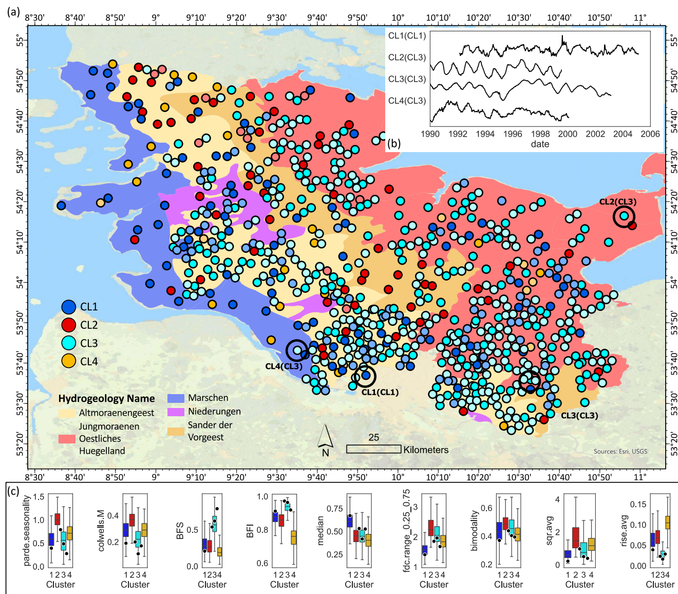
Figure 5 GWL dynamics patterns in the German federal state Schleswig-Holstein. (a) Cluster assignment to well locations and hydrogeology map of the German federal state Schleswig-Holstein (LfU-SH, 2003). Overlapping well markers are jittered at a minimum spacing of 500 meters and thus no longer represent the original well locations. Lighter cluster colors mark lower aquifer storeys. The cluster number in parentheses marks the true cluster from k-means clustering. (b) Exemplary time series of each cluster from the encircled well sites in (a). (c) Within-cluster variability of the example indices that each represent a component of the Heudorfer et al. 2019 typology from Fig. 3 plotted with indices values (dots) of the encircled well sites in (a) where the dots between CL2 and CL3 and CL4 and CL3 mark the wells that have the highest probability for CL2 and CL4 in the RF model but belong to CL3 according to the indices (see Fig. C5 for within-cluster variability for all indices that are plotted together with indices values of the selected well sites).
