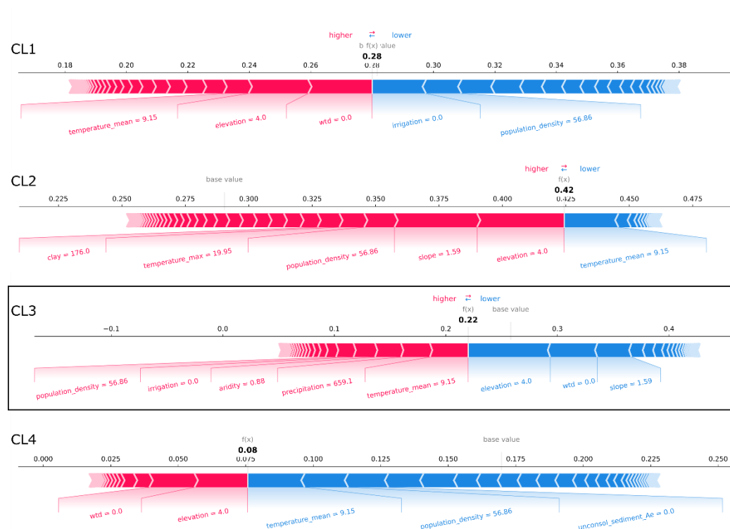
615 Figure E5 SHAP force plots explaining the prediction of the CL3 exemplary well site from the case study region in northern Germany (Fig. 5a) (from top to bottom: CL1, CL2, CL3, and CL4) that is confused with CL2. At this well site, the probability that CL2 is predicted is the largest in the case study (test dataset). The average scores of all classifications made by the Random Forest model for the training dataset are 0.28, 0.29, 0.26, and 0.17 respectively (base values). The model's probability scores for predicting the clusters at the exemplary well site (bold printed numbers) sum up to 100%. Features that are important for the respective predictions 620 are displayed with their values. Their importance and effect can be assessed by the SHAP values visualized by bar length and color (i.e. the larger the feature's share of the bar the more important; red represents rejecting effect and blue represents supporting effect).
