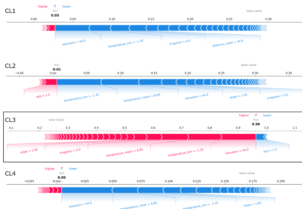
Figure E6 SHAP force plots explaining the correct prediction of the CL3 exemplary well site from the case study region in northern Germany (Fig. 5a) (from top to bottom: CL1, CL2, CL3, and CL4). At this well site, the probability that CL3 is predicted is the largest in the case study (test dataset). The average scores of all classifications made by the Random Forest model for the training dataset are 0.28, 0.29, 0.26, and 0.17 respectively (base values). The model's probability scores for predicting the clusters at the exemplary well site (bold printed numbers) sum up to 100%. Features that are important for the respective predictions are displayed with their values. Their importance and effects can be assessed by the SHAP values visualized by bar length and color (i.e. the larger the feature's share of the bar the more important; red represents rejecting effect and blue represents supporting effect).
