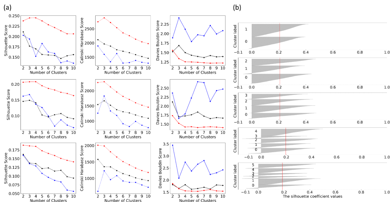
Figure C2 Evaluation metrics – Silhouette (Rousseeuw, 1987), Calinski-Harabasz (Caliński and Harabasz, 1974) and Davies-Bouldin (Davies and Bouldin, 1979) – used to find the best cluster separation. The Silhouette score ranges from -1 to 1, where a higher value
