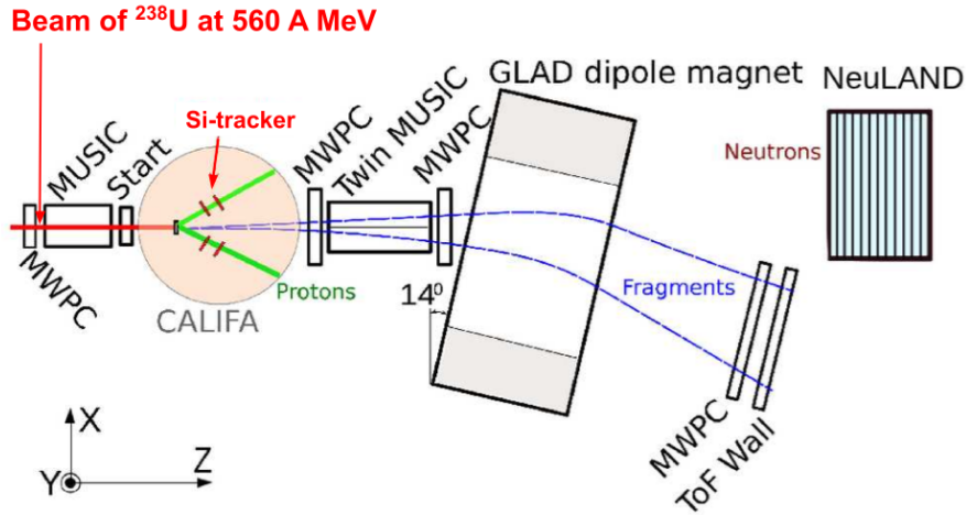
Figure 1: Schematic view of the experimental setup used in the present work to study quasi-free (p,2p) induced fission reactions.
